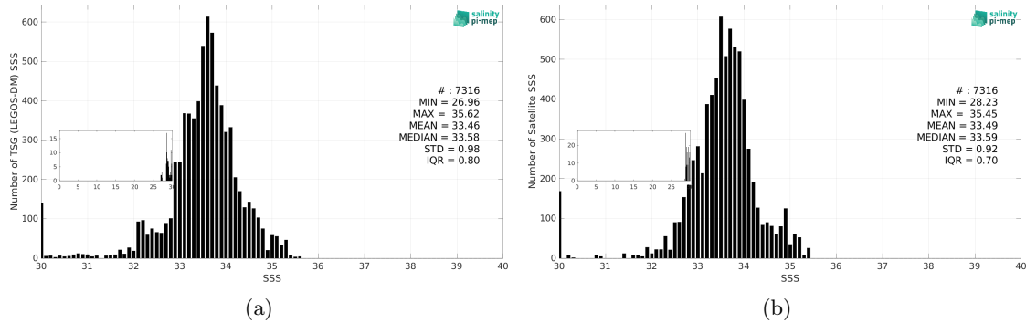
Figure 3: Histograms of SSS from TSG (LEGOS-DM) (a) and SMOS SSS L3 v332 - 9 Days (CATDS-CPDC) (b) considering all match-up pairs per bins of 0.1 over the Ganga and Brahmaputra river plumes Pi-MEP region and for the full satellite product period.
