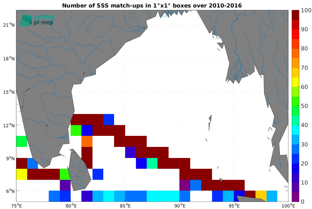
Figure 5: Number of SSS match-ups between TSG (LEGOS-DM) SSS and the SMOS SSS L3 v332 - 9 Days (CATDS-CPDC) SSS product for the Ganga and Brahmaputra river plumes Pi-MEP region over 1°×1° boxes and for the full satellite product period.
