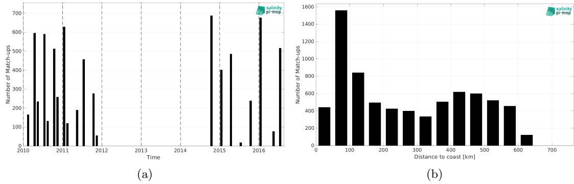
Figure 2: Number of match-ups between TSG (LEGOS-DM) and SMOS SSS L3 v332 - 9 Days (CATDS-CPDC) SSS as a function of time (a) and as function of the distance to coast (b) over the Ganga and Brahmaputra river plumes Pi-MEP region and for the full satellite product period.
