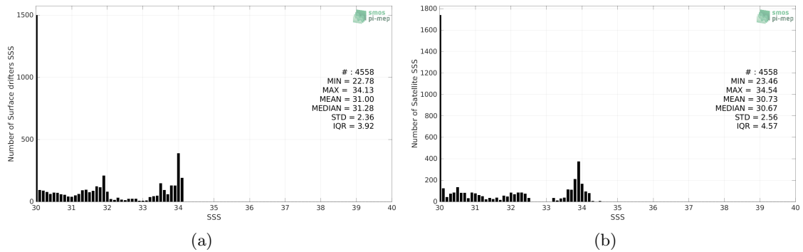
Figure 2: Histograms of SSS from Surface drifters (a) and SMOS SSS L3 v332 - 9 Days (CATDS-CPDC) (b) considering all match-up pairs per bins of 0.1 over the Ganga and Brahmaputra river plumes Pi-MEP region and for the full satellite product period.
