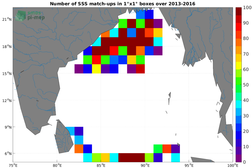
Figure 3: Number of SSS match-ups between Surface drifters SSS and the SMOS SSS L3 v332 - 9 Days (CATDS-CPDC) SSS product for the Ganga and Brahmaputra river plumes Pi-MEP region over 1°x1° boxes and for the full satellite product period.
