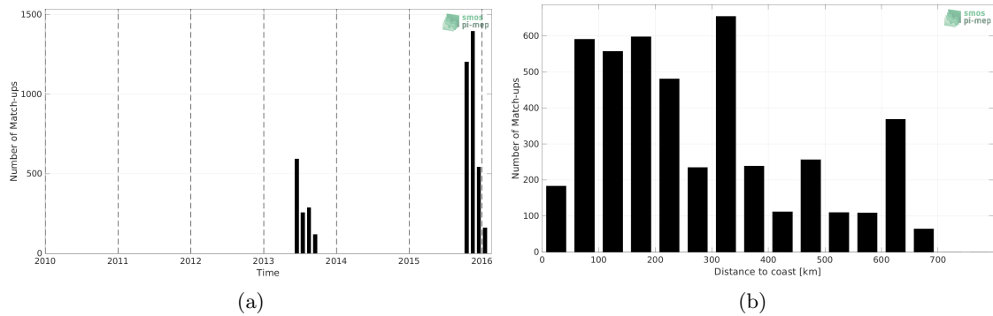
Figure 1: Number of match-ups between Surface drifters and SMOS SSS L3 v332 - 9 Days (CATDS-CPDC) SSS as a function of time (a) and as function of the distance to coast (b) over the Ganga and Brahmaputra river plumes Pi-MEP region and for the full satellite product period.
