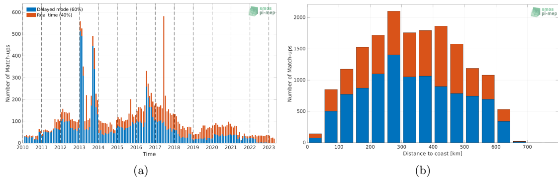
Figure 1: Number of match-ups between Argo and SMOS SSS L3 v332 - 9 Days (CATDS-CPDC) SSS as a function of time (a) and as function of the distance to coast (b) over the Ganga and Brahmaputra river plumes Pi-MEP region and for the full satellite product period.
