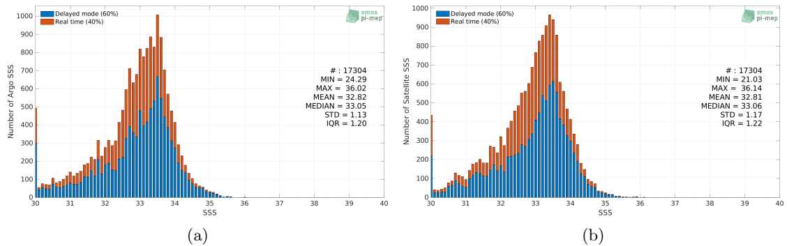
Figure 2: Histograms of SSS from Argo (a) and SMOS SSS L3 v332 - 9 Days (CATDS-CPDC) (b) considering all match-up pairs per bins of 0.1 over the Ganga and Brahmaputra river plumes Pi-MEP region and for the full satellite product period.
