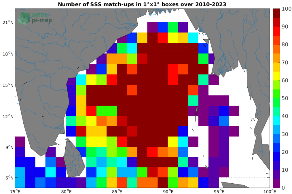
Figure 4: Number of SSS match-ups between Argo SSS and the SMOS SSS L3 v332 - 9 Days (CATDS-CPDC) SSS product for the Ganga and Brahmaputra river plumes Pi-MEP region over 1^\circ \times 1^\circ boxes and for the full satellite product period.
