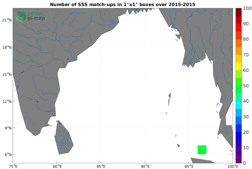
Figure 4: Number of SSS match-ups between TSG (SAMOS) SSS and the SMOS SSS L2Q v331 - 0.25 Deg (CATDS-CPDC) SSS product for the Ganga and Brahmaputra river plumes Pi-MEP region over 1^\circ \times 1^\circ boxes and for the full satellite product period.
