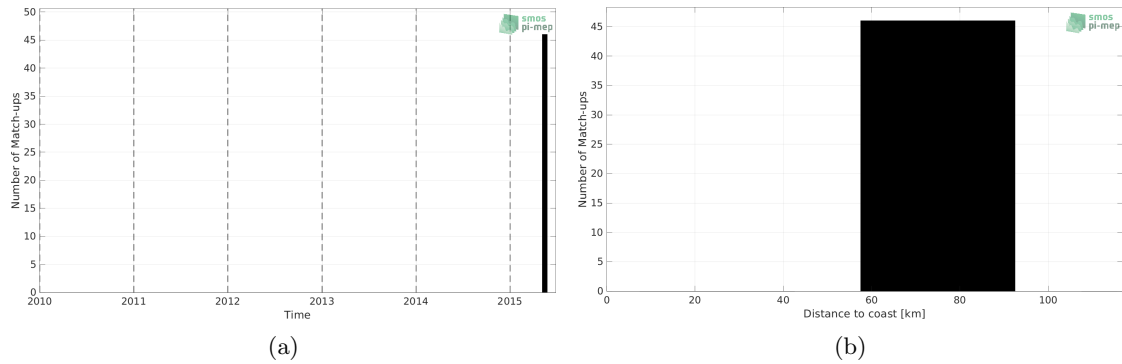
Figure 1: Number of match-ups between TSG (SAMOS) and SMOS SSS L2Q v331 - 0.25 Deg (CATDS-CPDC) SSS as a function of time (a) and as function of the distance to coast (b) over the Ganga and Brahmaputra river plumes Pi-MEP region and for the full satellite product period.
