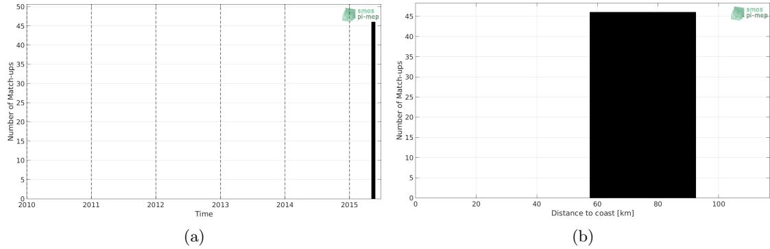
Figure 1: Number of match-ups between TSG (SAMOS) and SMOS SSS L2Q v330 - 0.25 Deg (CATDS-CPDC) SSS as a function of time (a) and as function of the distance to coast (b) over the Ganga and Brahmaputra river plumes Pi-MEP region and for the full satellite product period.
