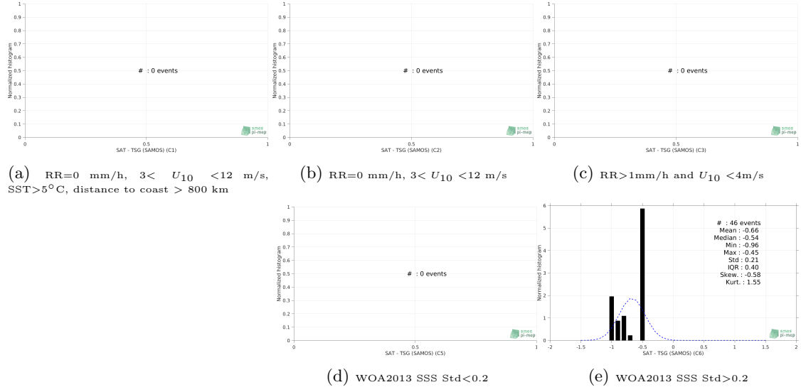
Figure 13: Normalized histogram of \Delta\text{SSS} (SMOS SSS L2Q v330 - 0.25 Deg (CATDS-CPDC) - TSG (SAMOS)) for 5 different subdatasets corresponding to: RR=0 mm/h, 3 < U_{10} < 12 m/s, SST > 5^\circ\text{C} , distance to coast > 800 km (a), RR=0 mm/h, 3 < U_{10} < 12 m/s (b), RR > 1\text{mm/h} and U_{10} < 4\text{m/s} (c), WOA2013 SSS Std < 0.2 (d), WOA2013 SSS Std > 0.2 (e).
