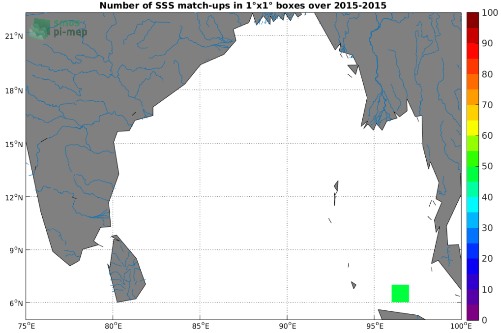
Figure 4: Number of SSS match-ups between TSG (SAMOS) SSS and the SMOS SSS L2Q v330 - 0.25 Deg (CATDS-CPDC) SSS product for the Ganga and Brahmaputra river plumes Pi-MEP region over 1^\circ \times 1^\circ boxes and for the full satellite product period.
