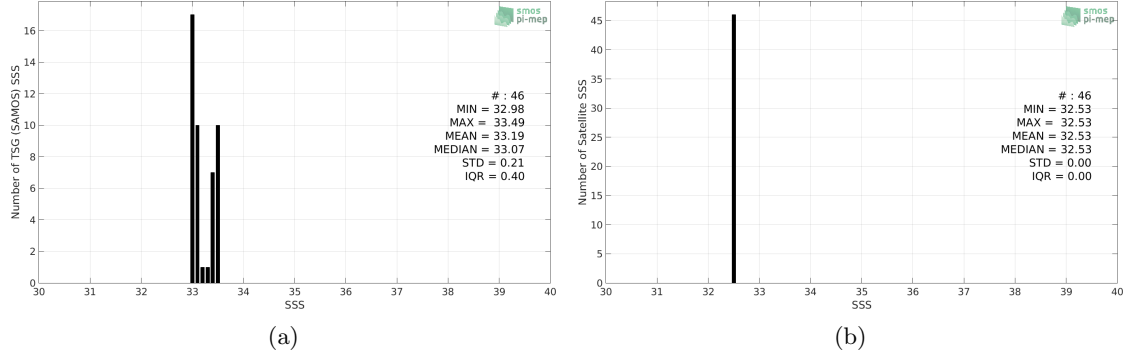
Figure 2: Histograms of SSS from TSG (SAMOS) (a) and SMOS SSS L2Q v330 - 0.25 Deg (CATDS-CPDC) (b) considering all match-up pairs per bins of 0.1 over the Ganga and Brahmaputra river plumes Pi-MEP region and for the full satellite product period.
