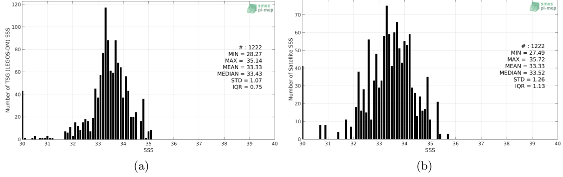
Figure 2: Histograms of SSS from TSG (LEGOS-DM) (a) and SMOS SSS L2Q v330 - 0.25 Deg (CATDS-CPDC) (b) considering all match-up pairs per bins of 0.1 over the Ganga and Brahmaputra river plumes Pi-MEP region and for the full satellite product period.
