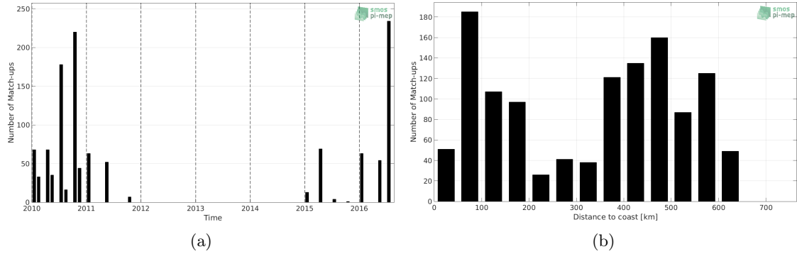
Figure 1: Number of match-ups between TSG (LEGOS-DM) and SMOS SSS L2Q v330 - 0.25 Deg (CATDS-CPDC) SSS as a function of time (a) and as function of the distance to coast (b) over the Ganga and Brahmaputra river plumes Pi-MEP region and for the full satellite product period.
