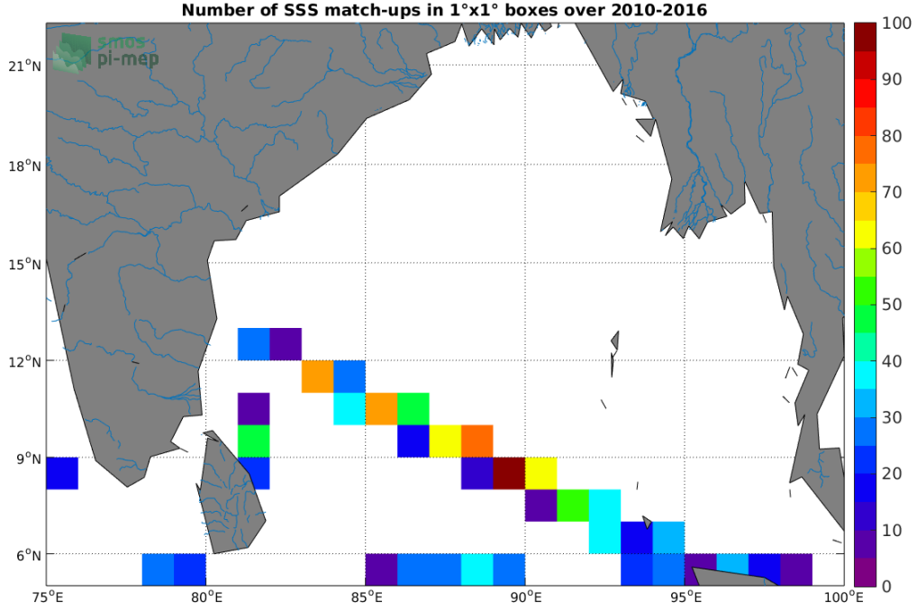
Figure 4: Number of SSS match-ups between TSG (LEGOS-DM) SSS and the SMOS SSS L2Q v330 - 0.25 Deg (CATDS-CPDC) SSS product for the Ganga and Brahmaputra river plumes Pi-MEP region over 1^\circ \times 1^\circ boxes and for the full satellite product period.
