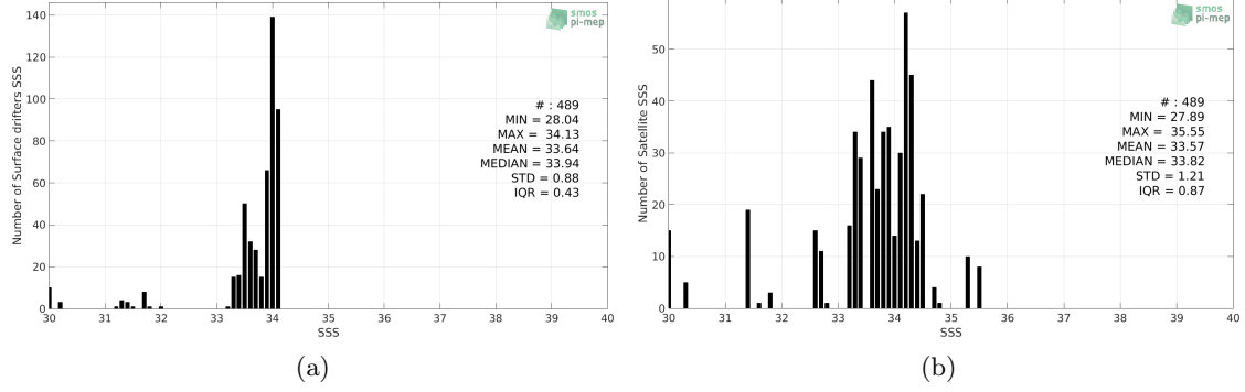
Figure 2: Histograms of SSS from Surface drifters (a) and SMOS SSS L2Q v330 - 0.25 Deg (CATDS-CPDC) (b) considering all match-up pairs per bins of 0.1 over the Ganga and Brahmaputra river plumes Pi-MEP region and for the full satellite product period.
