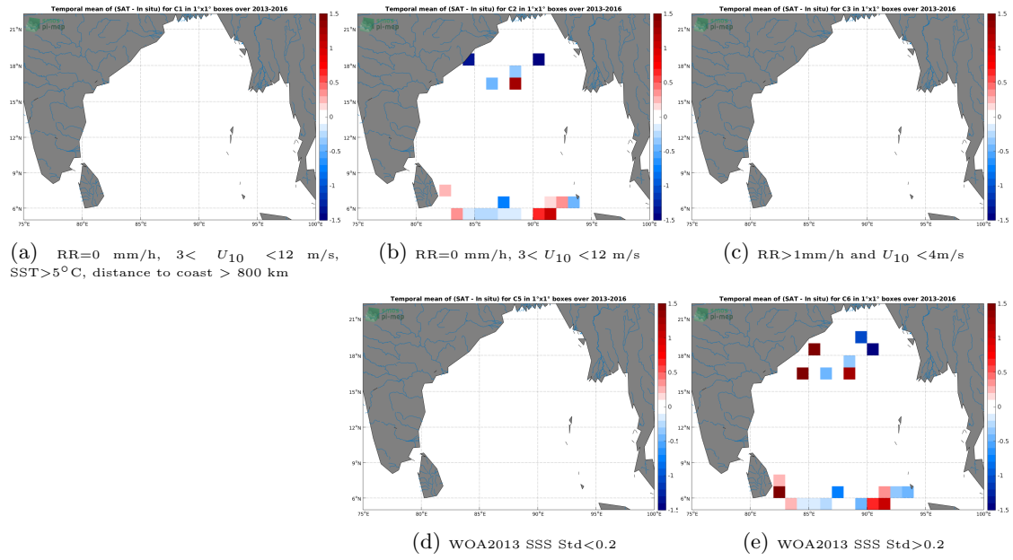
Figure 11: Temporal mean gridded over spatial boxes of size 1^\circ \times 1^\circ of \Delta\text{SSS} (SMOS SSS L2Q v330 - 0.25 Deg (CATDS-CPDC) - Surface drifters) for 5 different subdatasets corresponding to: RR=0 mm/h, 3 < U_{10} < 12 m/s, SST >5^\circ\text{C} , distance to coast > 800 km (a), RR=0 mm/h, 3 < U_{10} < 12 m/s (b), RR >1 mm/h and U_{10} < 4 m/s (c), WOA2013 SSS Std <0.2 (d), WOA2013 SSS Std >0.2 (e).
