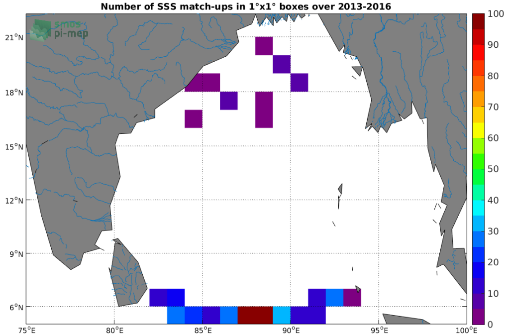
Figure 3: Number of SSS match-ups between Surface drifters SSS and the SMOS SSS L2Q v330 - 0.25 Deg (CATDS-CPDC) SSS product for the Ganga and Brahmaputra river plumes Pi-MEP region over 1^\circ \times 1^\circ boxes and for the full satellite product period.
