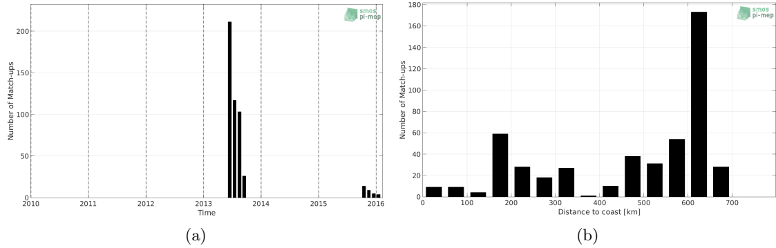
Figure 1: Number of match-ups between Surface drifters and SMOS SSS L2Q v330 - 0.25 Deg (CATDS-CPDC) SSS as a function of time (a) and as function of the distance to coast (b) over the Ganga and Brahmaputra river plumes Pi-MEP region and for the full satellite product period.
