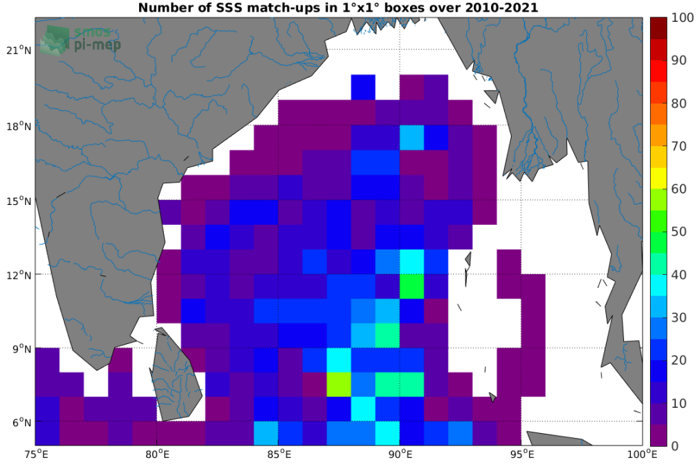
Figure 4: Number of SSS match-ups between Argo SSS and the SMOS SSS L2Q v330 - 0.25 Deg (CATDS-CPDC) SSS product for the Ganga and Brahmaputra river plumes Pi-MEP region over 1^\circ \times 1^\circ boxes and for the full satellite product period.
