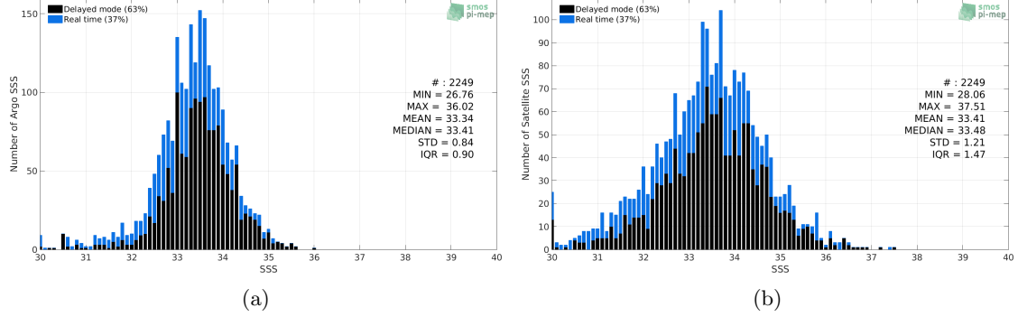
Figure 2: Histograms of SSS from Argo (a) and SMOS SSS L2Q v330 - 0.25 Deg (CATDS-CPDC) (b) considering all match-up pairs per bins of 0.1 over the Ganga and Brahmaputra river plumes Pi-MEP region and for the full satellite product period.
