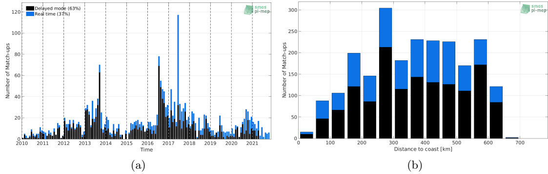
Figure 1: Number of match-ups between Argo and SMOS SSS L2Q v330 - 0.25 Deg (CATDS-CPDC) SSS as a function of time (a) and as function of the distance to coast (b) over the Ganga and Brahmaputra river plumes Pi-MEP region and for the full satellite product period.
