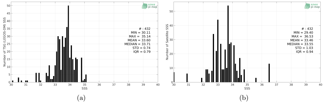
Figure 2: Histograms of SSS from TSG (LEGOS-DM) (a) and SMOS SSS L2Q v321 - 0.25 Deg (CATDS-CPDC) (b) considering all match-up pairs per bins of 0.1 over the Ganga and Brahmaputra river plumes Pi-MEP region and for the full satellite product period.
