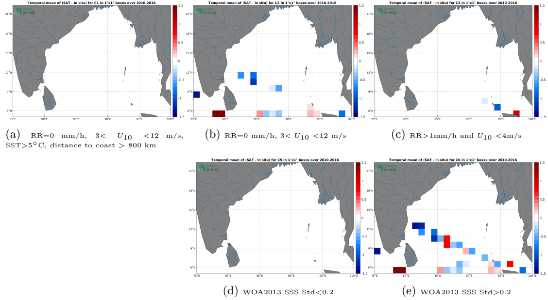
Figure 12: Temporal mean gridded over spatial boxes of size 1^{\circ}\times 1^{\circ} of \Delta\text{SSS} (SMOS SSS L2Q v321 - 0.25 Deg (CATDS-CPDC) - TSG (LEGOS-DM)) for 5 different subdatasets corresponding to: RR=0 mm/h, 3 < U_{10} < 12 m/s, SST > 5^{\circ}\text{C} , distance to coast > 800 km (a), RR=0 mm/h, 3 < U_{10} < 12 m/s (b), RR > 1 mm/h and U_{10} < 4 m/s (c), WOA2013 SSS Std < 0.2 (d), WOA2013 SSS Std > 0.2 (e).
