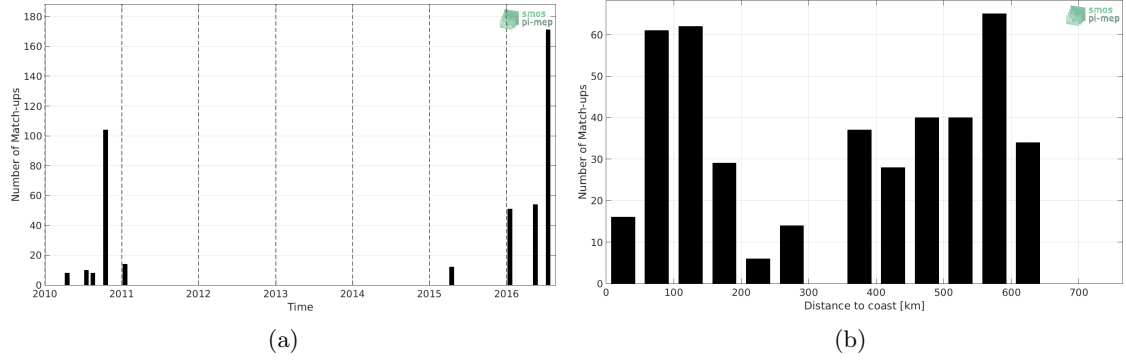
Figure 1: Number of match-ups between TSG (LEGOS-DM) and SMOS SSS L2Q v321 - 0.25 Deg (CATDS-CPDC) SSS as a function of time (a) and as function of the distance to coast (b) over the Ganga and Brahmaputra river plumes Pi-MEP region and for the full satellite product period.
