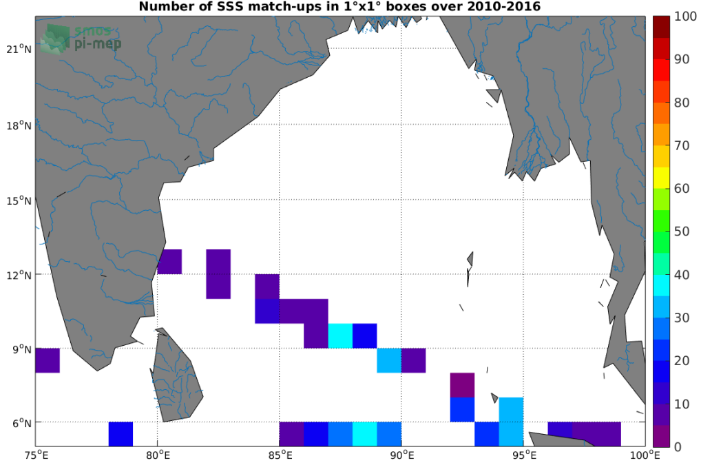
Figure 4: Number of SSS match-ups between TSG (LEGOS-DM) SSS and the SMOS SSS L2Q v321 - 0.25 Deg (CATDS-CPDC) SSS product for the Ganga and Brahmaputra river plumes Pi-MEP region over 1^\circ \times 1^\circ boxes and for the full satellite product period.
