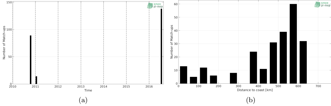
Figure 1: Number of match-ups between TSG-LEGOS-DM and SMOS-L3-CATDS-CPDC-V321-L2Q SSS as a function of time (a) and as function of the distance to coast (b) over the Ganga and Brahmaputra river plumes Pi-MEP region and for the full satellite product period.
