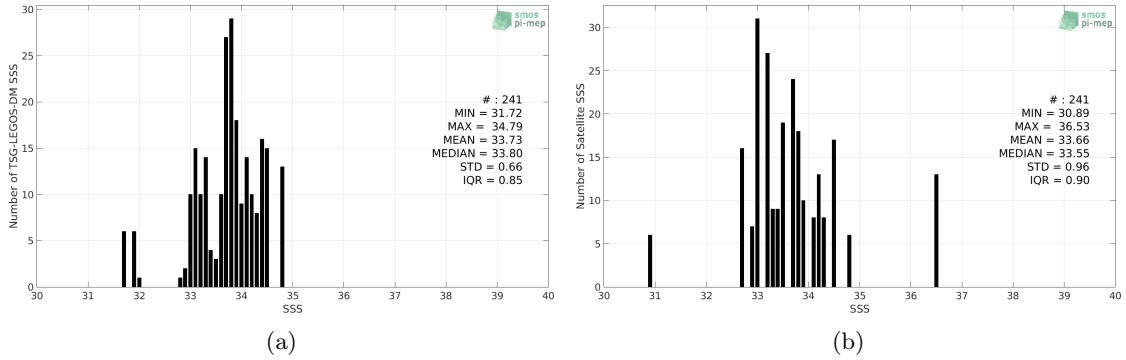
Figure 2: Histograms of SSS from TSG-LEGOS-DM (a) and SMOS-L3-CATDS-CPDC-V321-L2Q (b) considering all match-up pairs per bins of 0.1 over the Ganga and Brahmaputra river plumes Pi-MEP region and for the full satellite product period.
