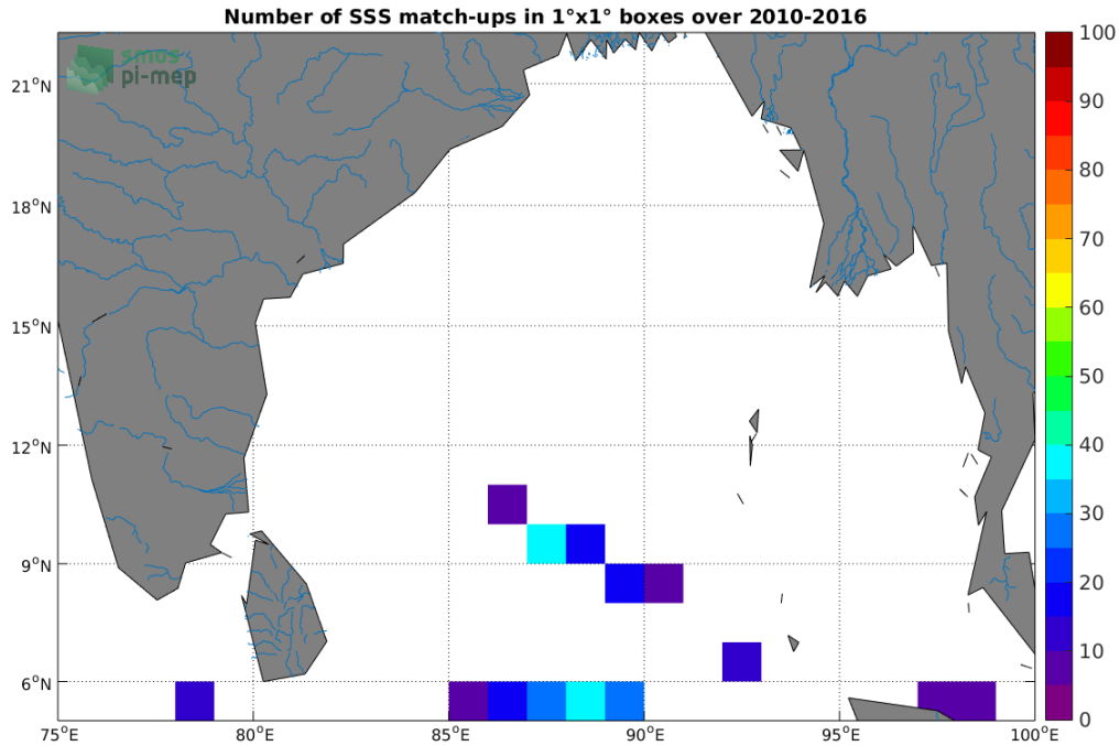
Figure 4: Number of SSS match-ups between TSG-LEGOS-DM SSS and the SMOS-L3-CATDS-CPDC-V321-L2Q SSS product for the Ganga and Brahmaputra river plumes Pi-MEP region over 1°x1° boxes and for the full satellite product period.
