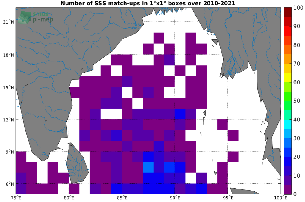
Figure 4: Number of SSS match-ups between Argo SSS and the SMOS SSS L2Q v321 - 0.25 Deg (CATDS-CPDC) SSS product for the Ganga and Brahmaputra river plumes Pi-MEP region over 1^\circ \times 1^\circ boxes and for the full satellite product period.
