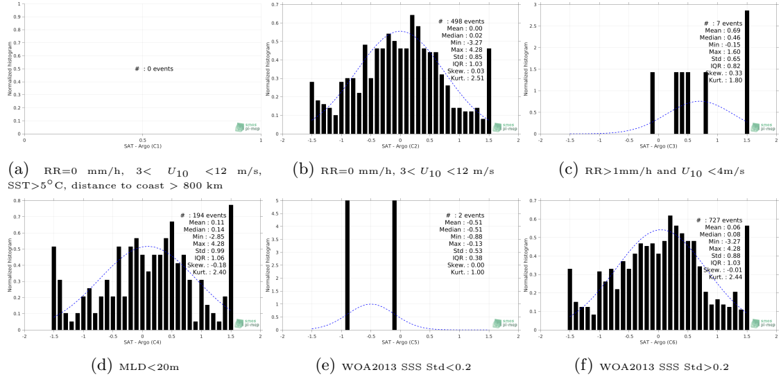
Figure 13: Normalized histogram of \Delta\text{SSS} (SMOS SSS L2Q v321 - 0.25 Deg (CATDS-CPDC) - Argo) for 6 different subdatasets corresponding to: RR=0 mm/h, 3 < U_{10} < 12 m/s, SST>5°C, distance to coast > 800 km (a), RR=0 mm/h, 3 < U_{10} < 12 m/s (b), RR>1mm/h and U_{10} < 4 m/s (c), MLD<20m (d), WOA2013 SSS Std<0.2 (e), WOA2013 SSS Std>0.2 (f).
