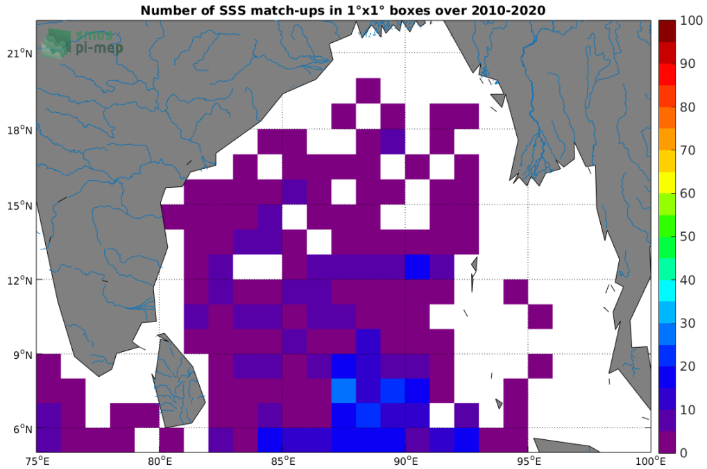
Figure 4: Number of SSS match-ups between Argo SSS and the SMOS SSS L2Q v321 - 0.25 Deg (CATDS-CPDC) SSS product for the Ganga and Brahmaputra river plumes Pi-MEP region over 1°x1° boxes and for the full satellite product period.
