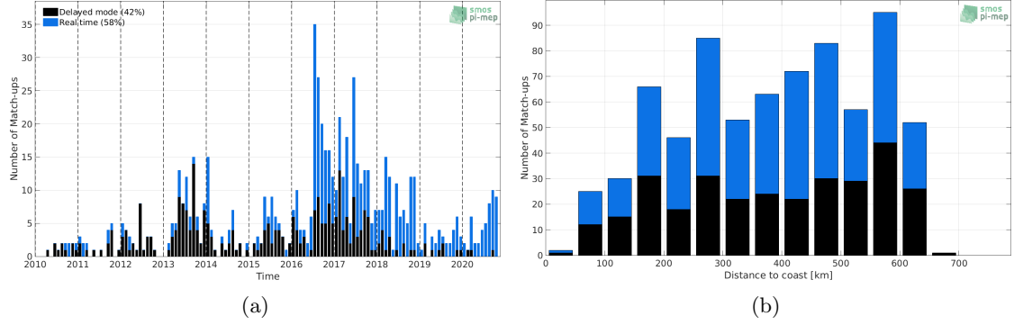
Figure 1: Number of match-ups between Argo and SMOS SSS L2Q v321 - 0.25 Deg (CATDS-CPDC) SSS as a function of time (a) and as function of the distance to coast (b) over the Ganga and Brahmaputra river plumes Pi-MEP region and for the full satellite product period.
