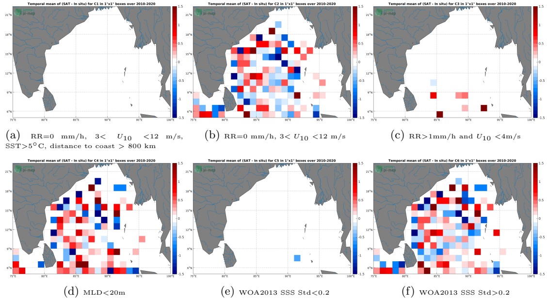
Figure 12: Temporal mean gridded over spatial boxes of size 1^\circ \times 1^\circ of \Delta SSS (SMOS SSS L2Q v321 - 0.25 Deg (CATDS-CPDC) - Argo) for 6 different subdatasets corresponding to: RR=0 mm/h, 3 < U_{10} < 12 m/s, SST >5^\circ\text{C} , distance to coast > 800 km (a), RR=0 mm/h, 3 < U_{10} < 12 m/s (b), RR >1 mm/h and U_{10} < 4 m/s (c),MLD <20 m (d),WOA2013 SSS Std <0.2 (e),WOA2013 SSS Std >0.2 (f).
