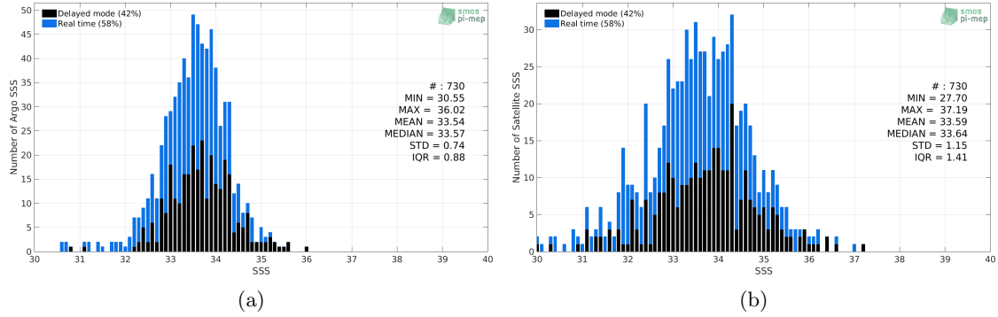
Figure 2: Histograms of SSS from Argo (a) and SMOS SSS L2Q v321 - 0.25 Deg (CATDS-CPDC) (b) considering all match-up pairs per bins of 0.1 over the Ganga and Brahmaputra river plumes Pi-MEP region and for the full satellite product period.
