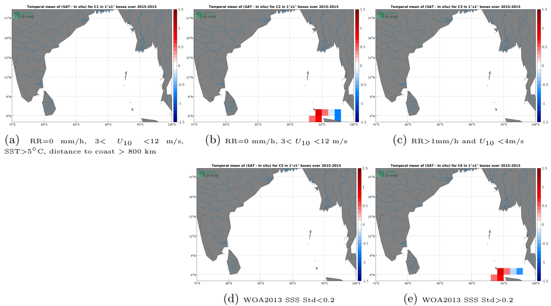
Figure 12: Temporal mean gridded over spatial boxes of size 1°x1° of \Delta SSS (SMOS SSS L3 v317 - Monthly - 25 km (CATDS-CPDC) - TSG (SAMOS)) for 5 different subdatasets corresponding to:RR=0 mm/h, 3 < U_{10} < 12 m/s, SST>5°C, distance to coast > 800 km (a), RR=0 mm/h, 3 < U_{10} < 12 m/s (b), RR>1mm/h and U_{10} < 4 m/s (c), WOA2013 SSS Std<0.2 (d), WOA2013 SSS Std>0.2 (e).
