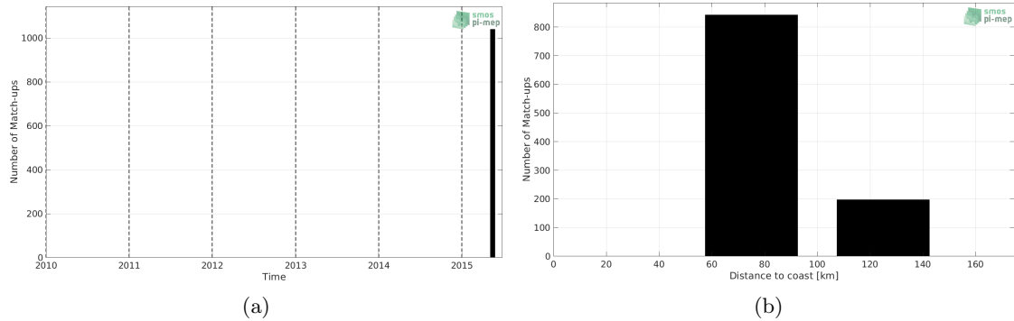
Figure 1: Number of match-ups between TSG (SAMOS) and SMOS SSS L3 v317 - Monthly - 25 km (CATDS-CPDC) SSS as a function of time (a) and as function of the distance to coast (b) over the Ganga and Brahmaputra river plumes Pi-MEP region and for the full satellite product period.
