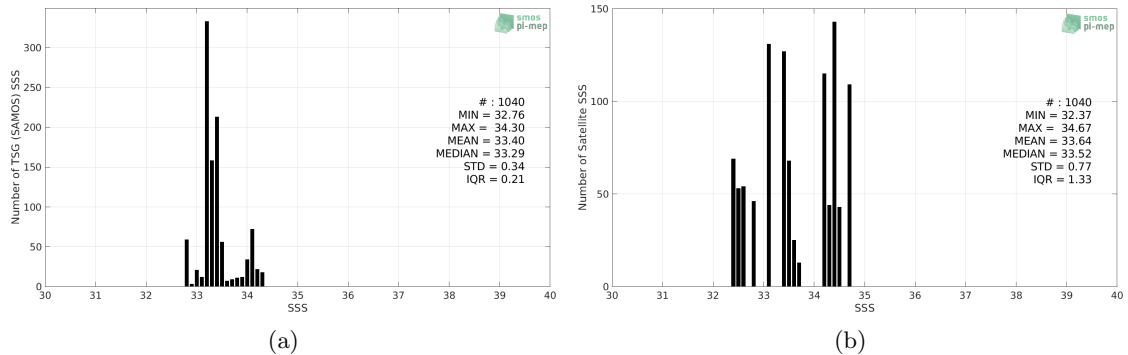
Figure 2: Histograms of SSS from TSG (SAMOS) (a) and SMOS SSS L3 v317 - Monthly - 25 km (CATDS-CPDC) (b) considering all match-up pairs per bins of 0.1 over the Ganga and Brahmaputra river plumes Pi-MEP region and for the full satellite product period.
