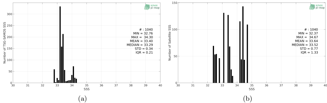
Figure 2: Histograms of SSS from TSG-SAMOS (a) and SMOS L3 v317 - Monthly - 25 km (CATDS-CPDC) (b) considering all match-up pairs per bins of 0.1 over the Ganga and Brahmaputra river plumes Pi-MEP region and for the full satellite product period.
