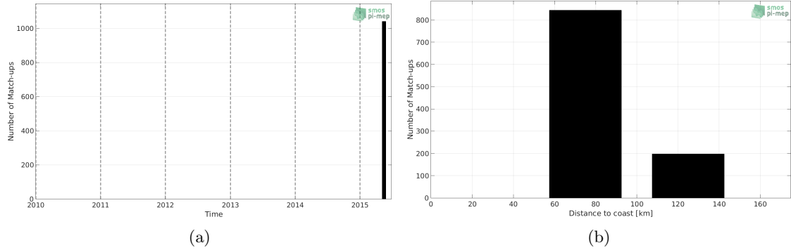
Figure 1: Number of match-ups between TSG-SAMOS and SMOS L3 v317 - Monthly - 25 km (CATDS-CPDC) SSS as a function of time (a) and as function of the distance to coast (b) over the Ganga and Brahmaputra river plumes Pi-MEP region and for the full satellite product period.
