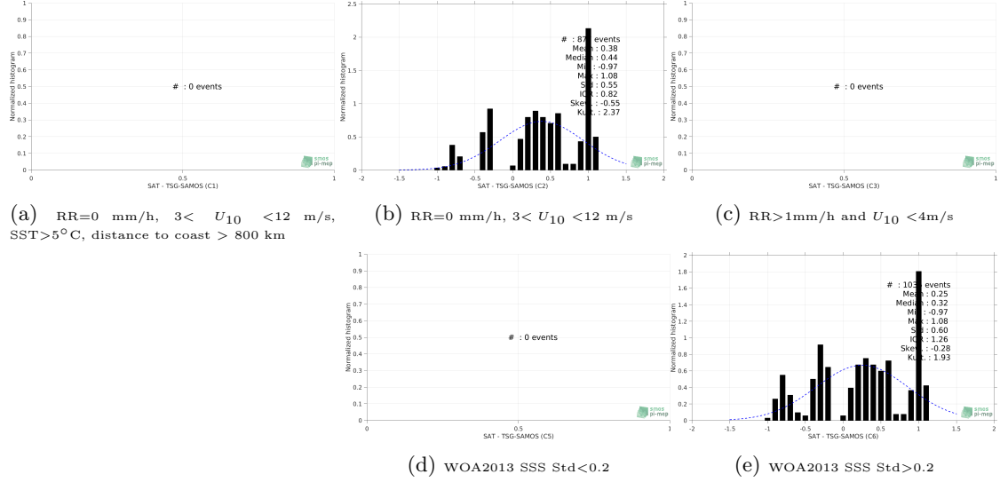
Figure 13: Normalized histogram of \Delta SSS (SMOS-L3-CATDS-CPDC-V317-MONTHLY-25KM - TSG-SAMOS) for 5 different subdatasets corresponding to: RR=0 mm/h, 3 < U_{10} < 12 m/s, SST >5^{\circ}\text{C} , distance to coast > 800 km (a), RR=0 mm/h, 3 < U_{10} < 12 m/s (b), RR >1 mm/h and U_{10} < 4 m/s (c), WOA2013 SSS Std <0.2 (d), WOA2013 SSS Std >0.2 (e).
