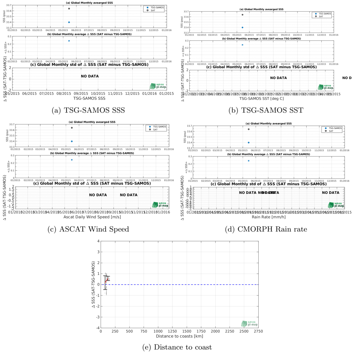
Figure 11: \Delta SSS (Satellite - TSG-SAMOS) sorted as function of TSG-SAMOS SSS a), TSG-SAMOS SST b), ASCAT Wind speed c), CMORPH rain rate d) and distance to coast (e). In all plots the mean and Std of \Delta SSS for each bin is indicated by the red curves and black vertical thick bars ( \pm 1 Std)
