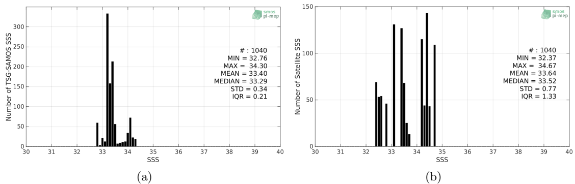
Figure 2: Histograms of SSS from TSG-SAMOS (a) and SMOS-L3-CATDS-CPDC-V317-MONTHLY-25KM (b) considering all match-up pairs per bins of 0.1 over the Ganga and Brahmaputra river plumes Pi-MEP region and for the full satellite product period.
