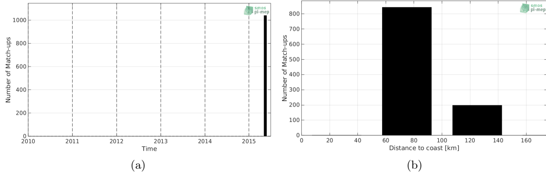
Figure 1: Number of match-ups between TSG-SAMOS and SMOS-L3-CATDS-CPDC-V317-MONTHLY-25KM SSS as a function of time (a) and as function of the distance to coast (b) over the Ganga and Brahmaputra river plumes Pi-MEP region and for the full satellite product period.
