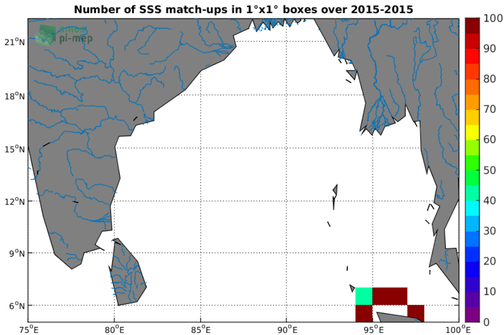
Figure 4: Number of SSS match-ups between TSG-SAMOS SSS and the SMOS-L3-CATDS-CPDC-V317-MONTHLY-25KM SSS product for the Ganga and Brahmaputra river plumes Pi-MEP region over 1^{\circ} \times 1^{\circ} boxes and for the full satellite product period.
