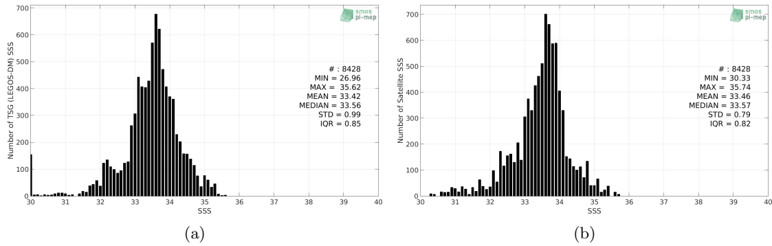
Figure 2: Histograms of SSS from TSG (LEGOS-DM) (a) and SMOS SSS L3 v317 - Monthly - 25 km (CATDS-CPDC) (b) considering all match-up pairs per bins of 0.1 over the Ganga and Brahmaputra river plumes Pi-MEP region and for the full satellite product period.
