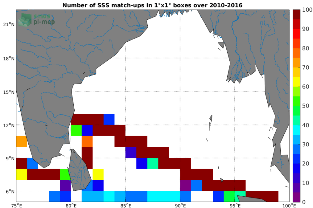
Figure 4: Number of SSS match-ups between TSG (LEGOS-DM) SSS and the SMOS SSS L3 v317 - Monthly - 25 km (CATDS-CPDC) SSS product for the Ganga and Brahmaputra river plumes Pi-MEP region over 1°x1° boxes and for the full satellite product period.
