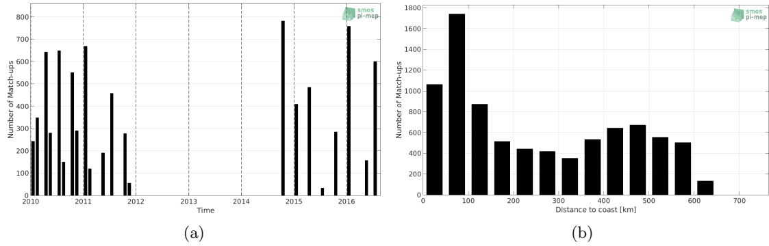
Figure 1: Number of match-ups between TSG (LEGOS-DM) and SMOS SSS L3 v317 - Monthly - 25 km (CATDS-CPDC) SSS as a function of time (a) and as function of the distance to coast (b) over the Ganga and Brahmaputra river plumes Pi-MEP region and for the full satellite product period.
