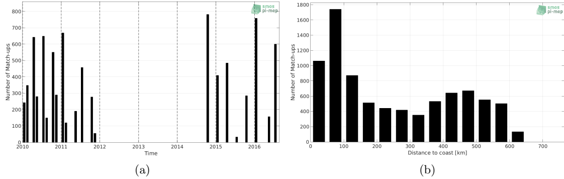
Figure 1: Number of match-ups between TSG-LEGOS-DM and SMOS L3 v317 - Monthly - 25 km (CATDS-CPDC) SSS as a function of time (a) and as function of the distance to coast (b) over the Ganga and Brahmaputra river plumes Pi-MEP region and for the full satellite product period.
