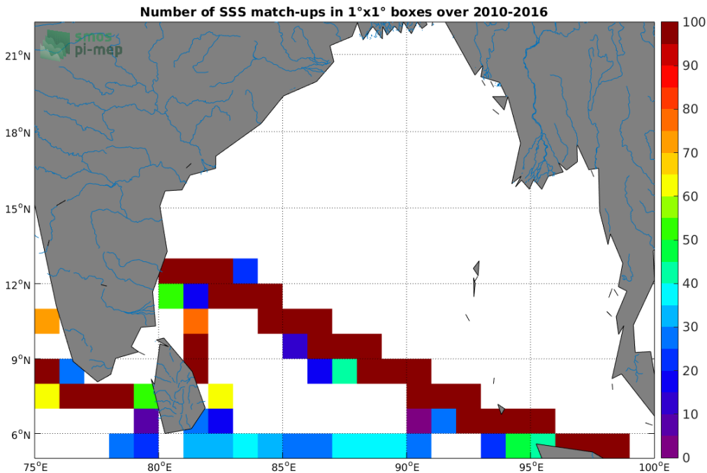
Figure 4: Number of SSS match-ups between TSG-LEGOS-DM SSS and the SMOS L3 v317 - Monthly - 25 km (CATDS-CPDC) SSS product for the Ganga and Brahmaputra river plumes Pi-MEP region over 1^\circ \times 1^\circ boxes and for the full satellite product period.
