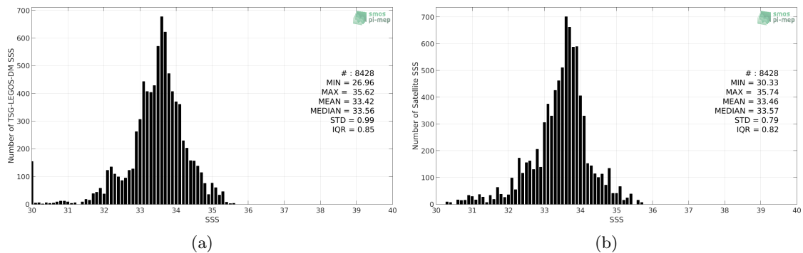
Figure 2: Histograms of SSS from TSG-LEGOS-DM (a) and SMOS L3 v317 - Monthly - 25 km (CATDS-CPDC) (b) considering all match-up pairs per bins of 0.1 over the Ganga and Brahmaputra river plumes Pi-MEP region and for the full satellite product period.
