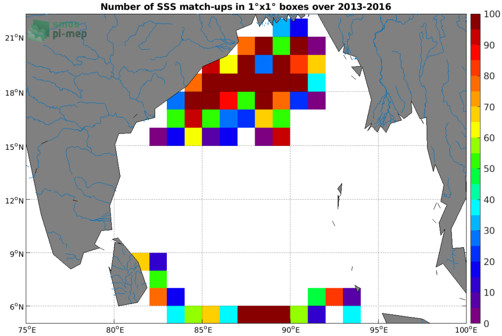
Figure 3: Number of SSS match-ups between Surface drifters SSS and the SMOS SSS L3 v317 - Monthly - 25 km (CATDS-CPDC) SSS product for the Ganga and Brahmaputra river plumes Pi-MEP region over 1^\circ \times 1^\circ boxes and for the full satellite product period.
