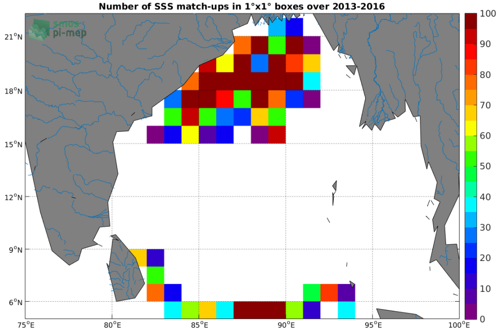
Figure 3: Number of SSS match-ups between Surface drifters SSS and the SMOS SSS L3 v317 - Monthly - 25 km (CATDS-CPDC) SSS product for the Ganga and Brahmaputra river plumes Pi-MEP region over 1°x1° boxes and for the full satellite product period.
