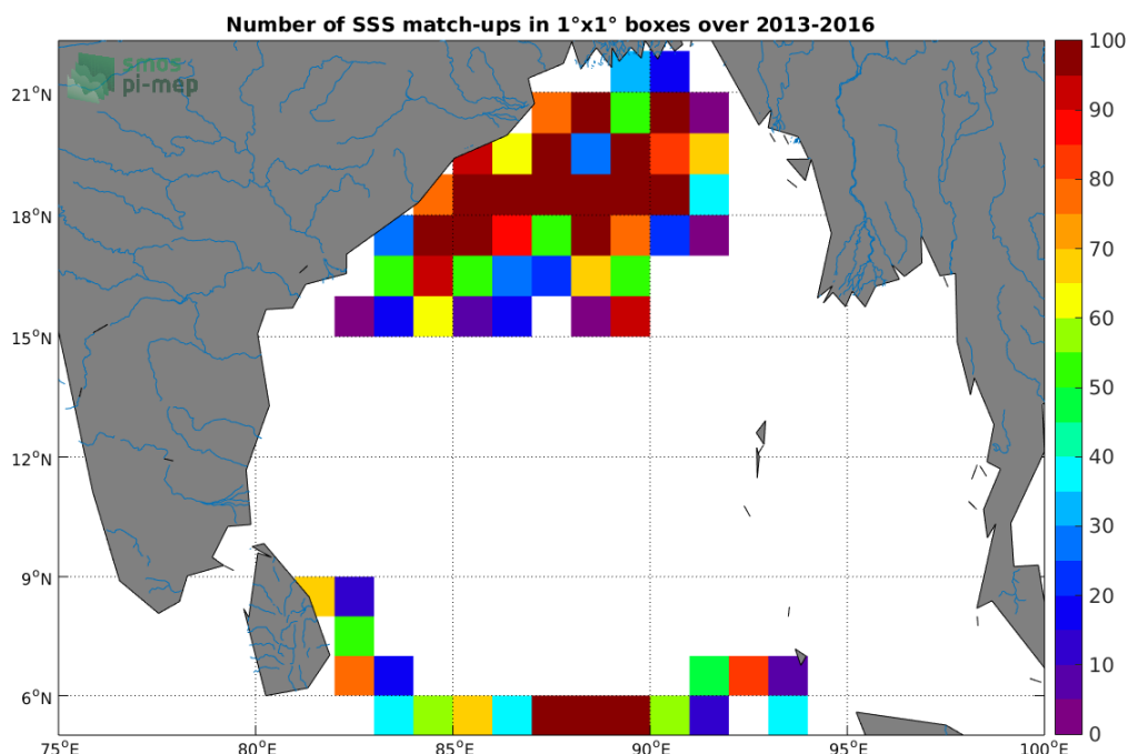
Figure 3: Number of SSS match-ups between Surface drifters SSS and the SMOS L3 v317 - Monthly - 25 km (CATDS-CPDC) SSS product for the Ganga and Brahmaputra river plumes Pi-MEP region over 1°x1° boxes and for the full satellite product period.
