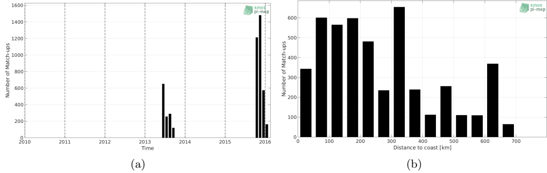
Figure 1: Number of match-ups between Surface drifters and SMOS L3 v317 - Monthly - 25 km (CATDS-CPDC) SSS as a function of time (a) and as function of the distance to coast (b) over the Ganga and Brahmaputra river plumes Pi-MEP region and for the full satellite product period.
