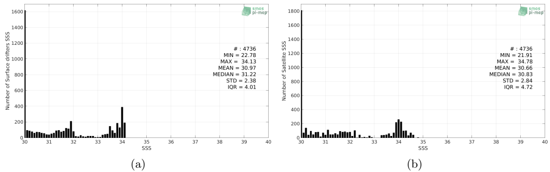
Figure 2: Histograms of SSS from Surface drifters (a) and SMOS L3 v317 - Monthly - 25 km (CATDS-CPDC) (b) considering all match-up pairs per bins of 0.1 over the Ganga and Brahmaputra river plumes Pi-MEP region and for the full satellite product period.
