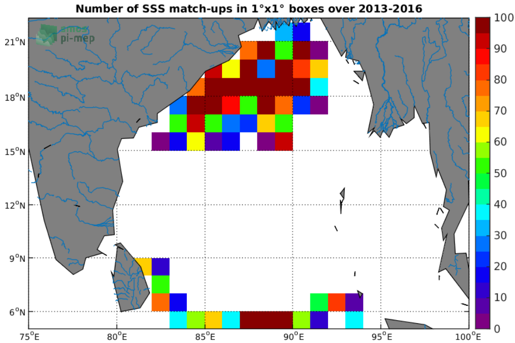
Figure 3: Number of SSS match-ups between Surface drifters SSS and the SMOS-L3-CATDS-CPDC-V317-MONTHLY-25KM SSS product for the Ganga and Brahmaputra river plumes Pi-MEP region over 1°x1° boxes and for the full satellite product period.
