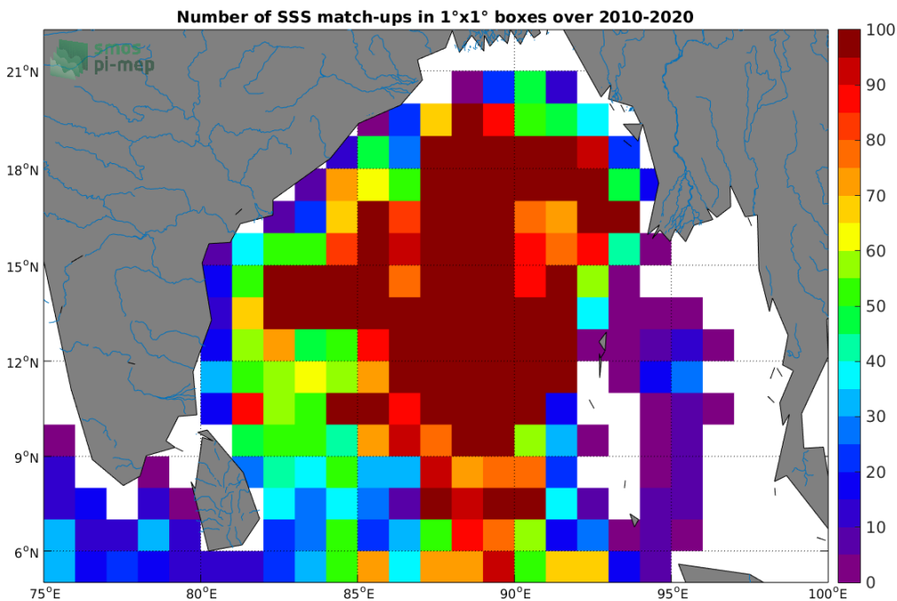
Figure 4: Number of SSS match-ups between Argos SSS and the SMOS L3 v317 - Monthly - 25 km (CATDS-CPDC) SSS product for the Ganga and Brahmaputra river plumes Pi-MEP region over 1°x1° boxes and for the full satellite product period.
