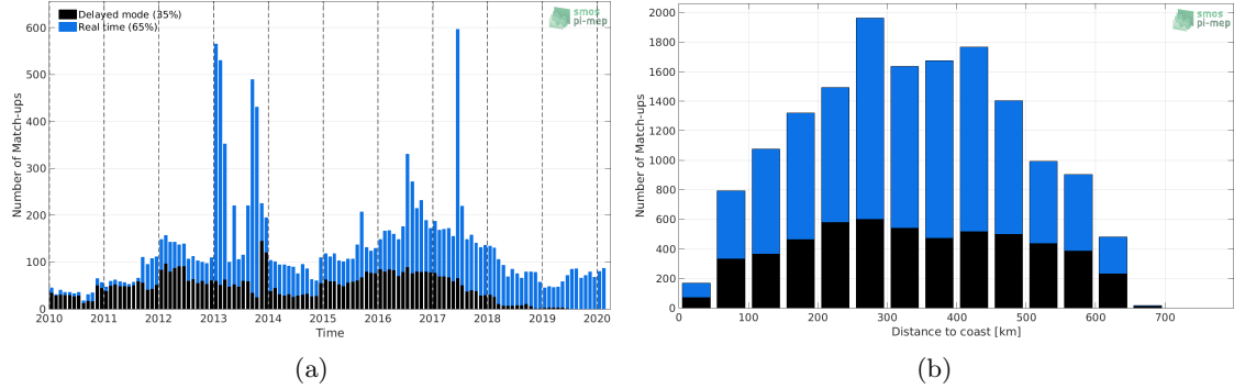
Figure 1: Number of match-ups between Argo and SMOS L3 v317 - Monthly - 25 km (CATDS-CPDC) SSS as a function of time (a) and as function of the distance to coast (b) over the Ganga and Brahmaputra river plumes Pi-MEP region and for the full satellite product period.
