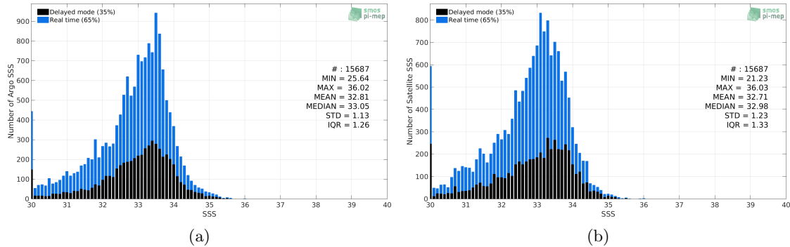
Figure 2: Histograms of SSS from Argo (a) and SMOS L3 v317 - Monthly - 25 km (CATDS-CPDC) (b) considering all match-up pairs per bins of 0.1 over the Ganga and Brahmaputra river plumes Pi-MEP region and for the full satellite product period.
