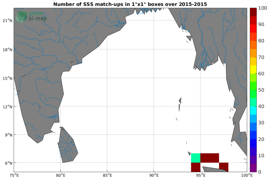
Figure 4: Number of SSS match-ups between TSG-SAMOS SSS and the SMOS-L3-CATDS-CPDC-V3-MONTHLY-25KM SSS product for the Ganga and Brahmaputra river plumes Pi-MEP region over 1^\circ \times 1^\circ boxes and for the full satellite product period.
