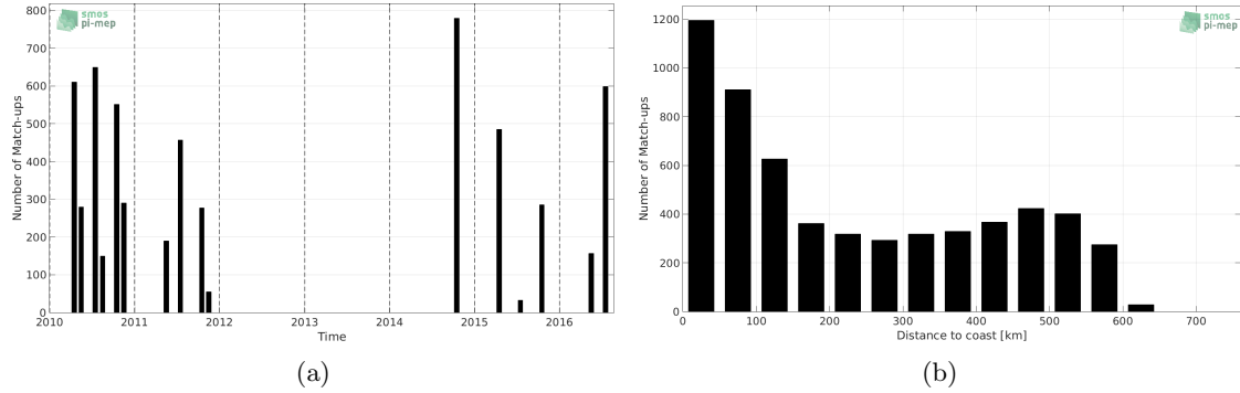
Figure 1: Number of match-ups between TSG-LEGOS-DM and SMOS-L3-CATDS-CPDC-V3-MONTHLY-25KM SSS as a function of time (a) and as function of the distance to coast (b) over the Ganga and Brahmaputra river plumes Pi-MEP region and for the full satellite product period.
