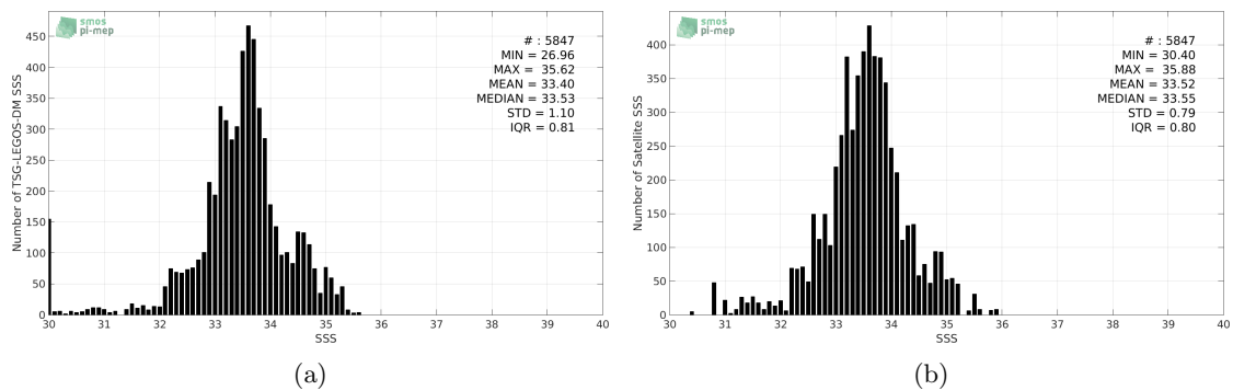
Figure 2: Histograms of SSS from TSG-LEGOS-DM (a) and SMOS-L3-CATDS-CPDC-V3-MONTHLY-25KM (b) considering all match-up pairs per bins of 0.1 over the Ganga and Brahmaputra river plumes Pi-MEP region and for the full satellite product period.
