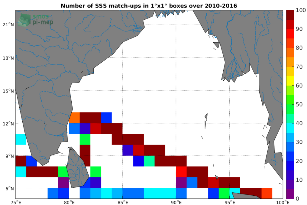
Figure 4: Number of SSS match-ups between TSG-LEGOS-DM SSS and the SMOS-L3-CATDS-CPDC-V3-MONTHLY-25KM SSS product for the Ganga and Brahmaputra river plumes Pi-MEP region over 1^\circ \times 1^\circ boxes and for the full satellite product period.
