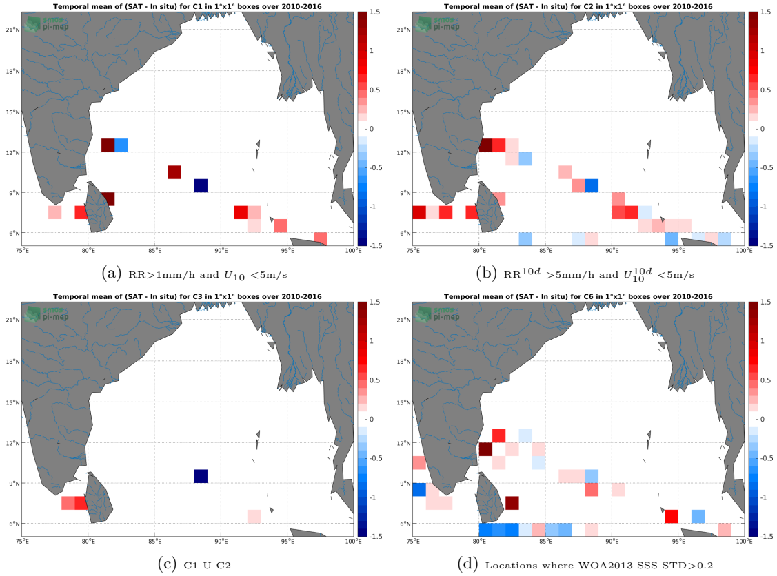
Figure 12: Temporal mean gridded over spatial boxes of size 1^\circ \times 1^\circ of \Delta SSS (SMOS-L3-CATDS-CPDC-V3-MONTHLY-25KM - TSG-LEGOS-DM) for 4 different subdatasets corresponding to: RR > 1\text{mm/h} and U_{10} < 5\text{m/s} (a), RR^{10d} > 5\text{mm/h} and U_{10}^{10d} < 5\text{m/s} (b), C1 U C2 (c), Locations where WOA2013 SSS STD > 0.2 (d).
