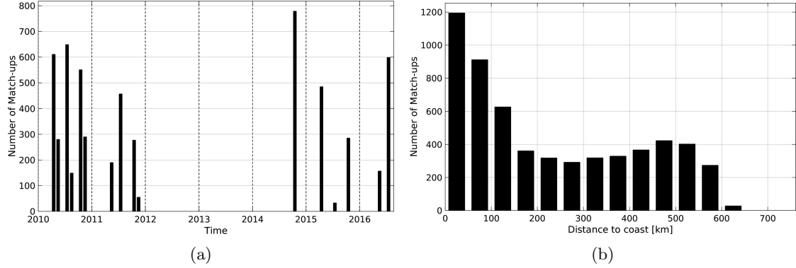
Figure 1: Number of match-ups between TSG-LEGOS-DM and SMOS-L3-CATDS-CPDC-V3-MONTHLY-25KM SSS as a function of time (a) and as function of the distance to coast (b) over the Ganga and Brahmaputra river plumes Pi-MEP region and for the full satellite product period.
