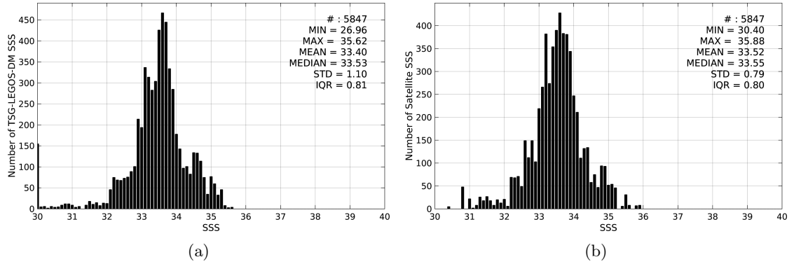
Figure 2: Histograms of SSS from TSG-LEGOS-DM (a) and SMOS-L3-CATDS-CPDC-V3-MONTHLY-25KM (b) considering all match-up pairs per bins of 0.1 over the Ganga and Brahmaputra river plumes Pi-MEP region and for the full satellite product period.
