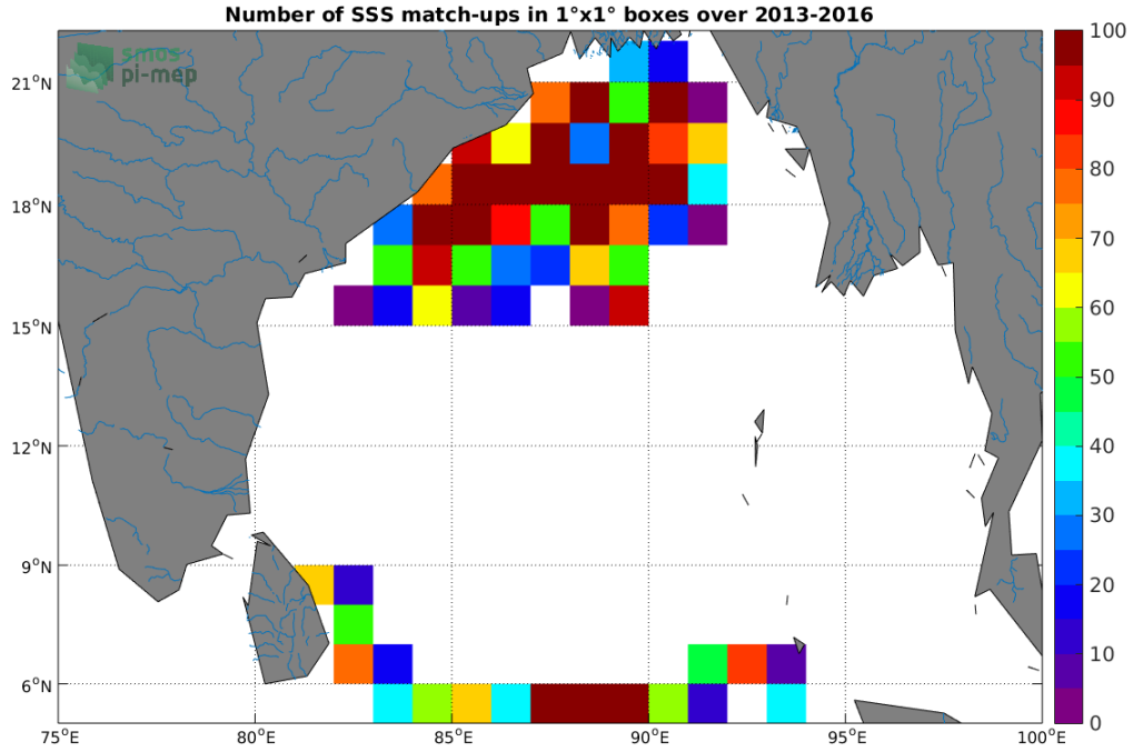
Figure 3: Number of SSS match-ups between Surface drifters SSS and the SMOS-L3-CATDS-CPDC-V3-MONTHLY-25KM SSS product for the Ganga and Brahmaputra river plumes Pi-MEP region over 1^\circ \times 1^\circ boxes and for the full satellite product period.
