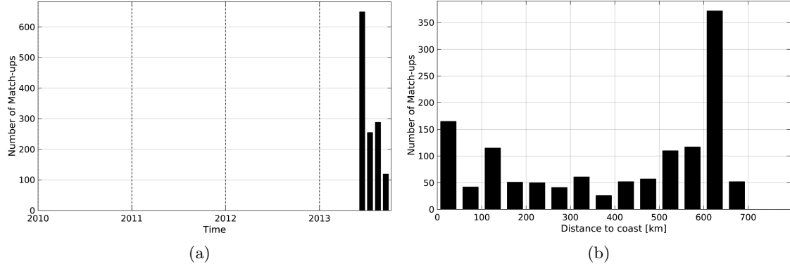
Figure 1: Number of match-ups between Surface drifters and SMOS-L3-CATDS-CPDC-V3-MONTHLY-25KM SSS as a function of time (a) and as function of the distance to coast (b) over the Ganga and Brahmaputra river plumes Pi-MEP region and for the full satellite product period.
