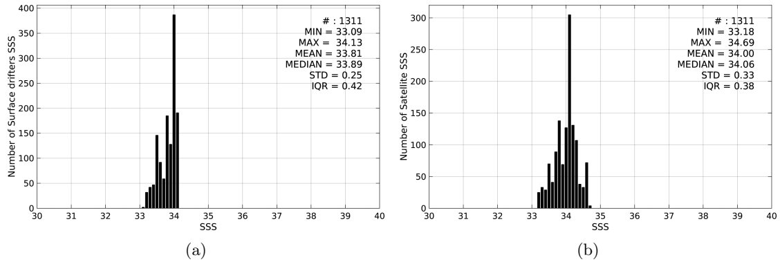
Figure 2: Histograms of SSS from Surface drifters (a) and SMOS-L3-CATDS-CPDC-V3-MONTHLY-25KM (b) considering all match-up pairs per bins of 0.1 over the Ganga and Brahmaputra river plumes Pi-MEP region and for the full satellite product period.
