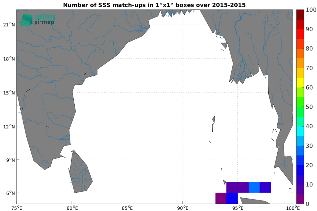
Figure 5: Number of SSS match-ups between TSG (SAMOS) SSS and the SMOS SSS L3 v2 - 9-Days (BEC) SSS product for the Ganga and Brahmaputra river plumes Pi-MEP region over 1^\circ \times 1^\circ boxes and for the full satellite product period.
