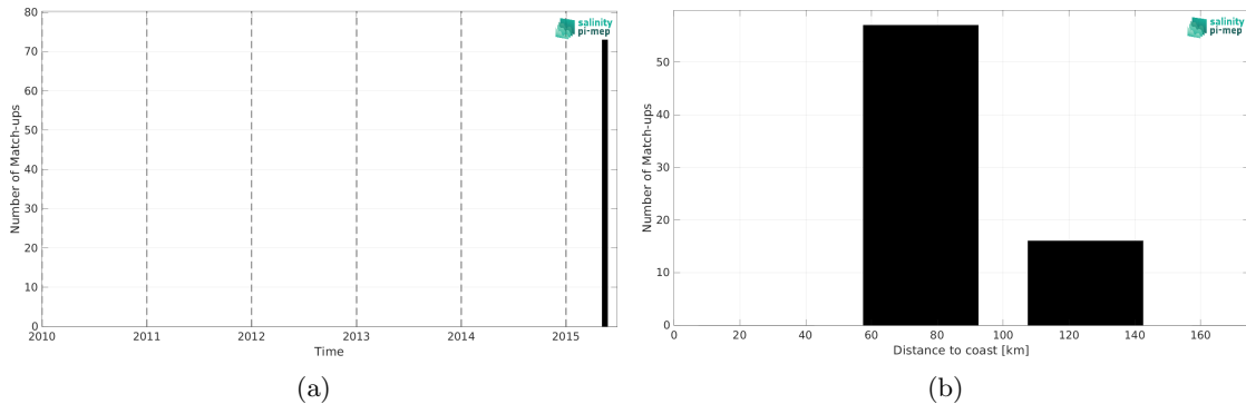
Figure 2: Number of match-ups between TSG (SAMOS) and SMOS SSS L3 v2 - 9-Days (BEC) SSS as a function of time (a) and as function of the distance to coast (b) over the Ganga and Brahmaputra river plumes Pi-MEP region and for the full satellite product period.
