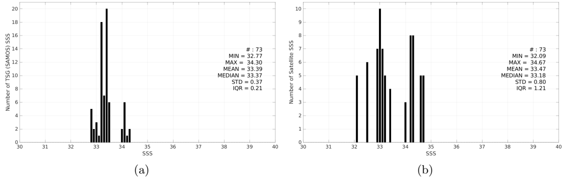
Figure 3: Histograms of SSS from TSG (SAMOS) (a) and SMOS SSS L3 v2 - 9-Days (BEC) (b) considering all match-up pairs per bins of 0.1 over the Ganga and Brahmaputra river plumes Pi-MEP region and for the full satellite product period.
