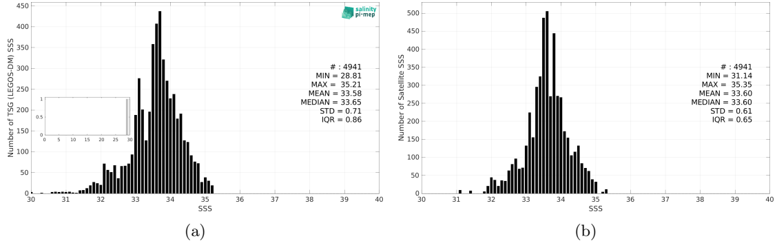
Figure 3: Histograms of SSS from TSG (LEGOS-DM) (a) and SMOS SSS L3 v2 - 9-Days (BEC) (b) considering all match-up pairs per bins of 0.1 over the Ganga and Brahmaputra river plumes Pi-MEP region and for the full satellite product period.
