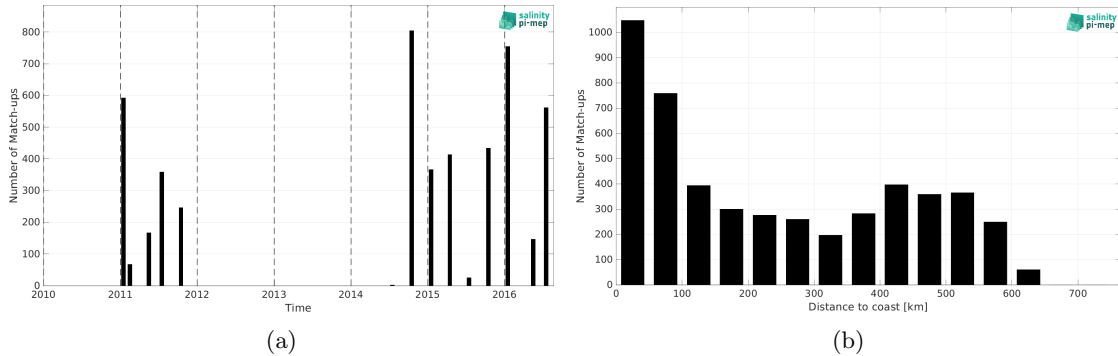
Figure 2: Number of match-ups between TSG (LEGOS-DM) and SMOS SSS L3 v2 - 9-Days (BEC) SSS as a function of time (a) and as function of the distance to coast (b) over the Ganga and Brahmaputra river plumes Pi-MEP region and for the full satellite product period.
