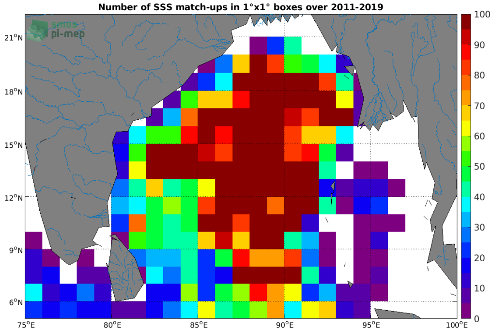
Figure 4: Number of SSS match-ups between Argo SSS and the SMOS SSS L3 v2 - 9-Days (BEC) SSS product for the Ganga and Brahmaputra river plumes Pi-MEP region over 1^{\circ} \times 1^{\circ} boxes and for the full satellite product period.
