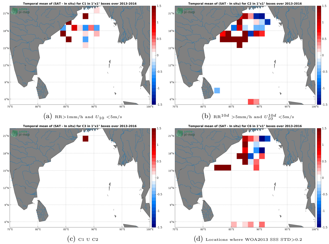
Figure 11: Temporal mean gridded over spatial boxes of size 1^\circ \times 1^\circ of \Delta SSS (SMOS-L3-BEC-OA-V1-9DAYS-0.25DEG - Surface drifters) for 4 different subdatasets corresponding to:RR >1 mm/h and U_{10} < 5 m/s (a), RR 10d > 5 mm/h and U_{10}^{10d} < 5 m/s (b), C1 U C2 (c),Locations where WOA2013 SSS STD >0.2 (d).
