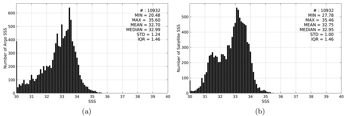
Figure 2: Histograms of SSS from Argo (a) and SMOS-L3-BEC-OA-V1-9DAYS-0.25DEG (b) considering all match-up pairs per bins of 0.1 over the Ganga and Brahmaputra river plumes Pi-MEP region and for the full satellite product period.
