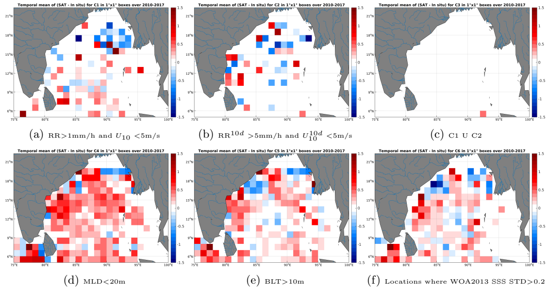
Figure 12: Temporal mean gridded over spatial boxes of size 1^\circ \times 1^\circ of \Delta SSS (SMOS-L3-BEC-OA-V1-9DAYS-0.25DEG - Argo) for 6 different subdatasets corresponding to: RR > 1\text{mm/h} and U_{10} < 5\text{m/s} (a), RR^{10d} > 5\text{mm/h} and U_{10}^{10d} < 5\text{m/s} (b), C1 U C2 (c), MLD < 20\text{m} (d), BLT > 10\text{m} (e), Locations where WOA2013 SSS STD > 0.2 (f).
