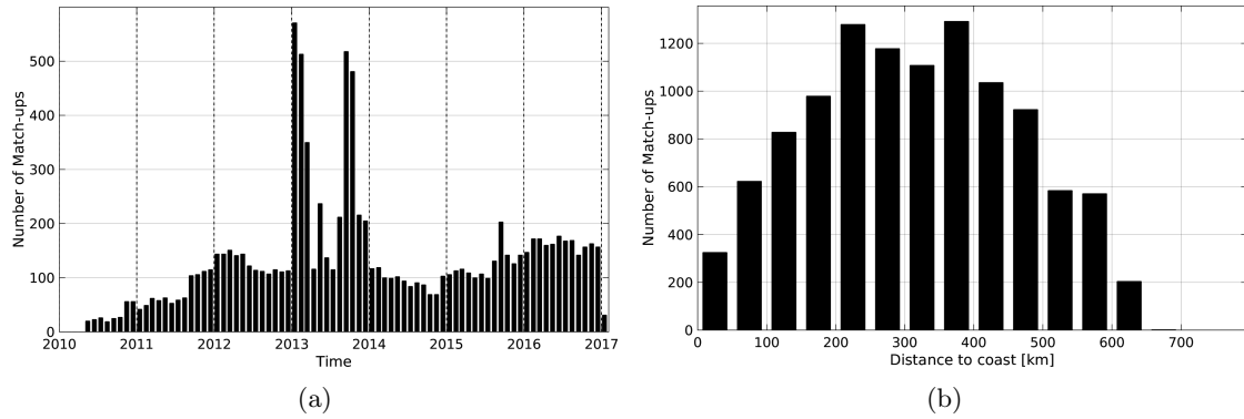
Figure 1: Number of match-ups between Argo and SMOS-L3-BEC-OA-V1-9DAYS-0.25DEG SSS as a function of time (a) and as function of the distance to coast (b) over the Ganga and Brahmaputra river plumes Pi-MEP region and for the full satellite product period.
