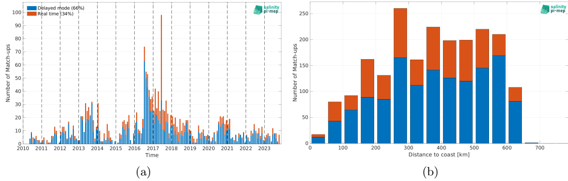
Figure 2: Number of match-ups between Argo and SMOS SSS L2 v700 (ESA) SSS as a function of time (a) and as function of the distance to coast (b) over the Ganga and Brahmaputra river plumes Pi-MEP region and for the full satellite product period.
