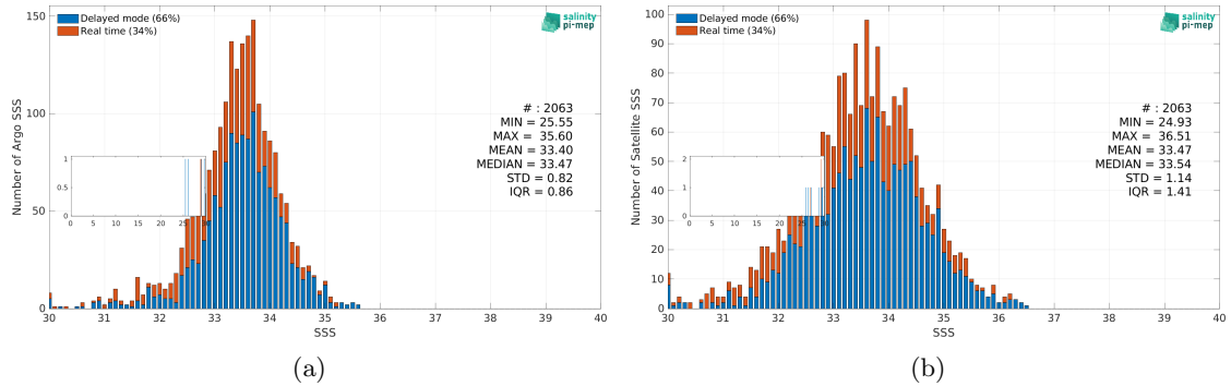
Figure 3: Histograms of SSS from Argo (a) and SMOS SSS L2 v700 (ESA) (b) considering all match-up pairs per bins of 0.1 over the Ganga and Brahmaputra river plumes Pi-MEP region and for the full satellite product period.
