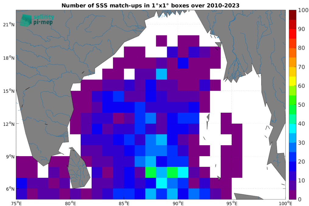
Figure 5: Number of SSS match-ups between Argo SSS and the SMOS SSS L2 v700 (ESA) SSS product for the Ganga and Brahmaputra river plumes Pi-MEP region over 1^\circ \times 1^\circ boxes and for the full satellite product period.
