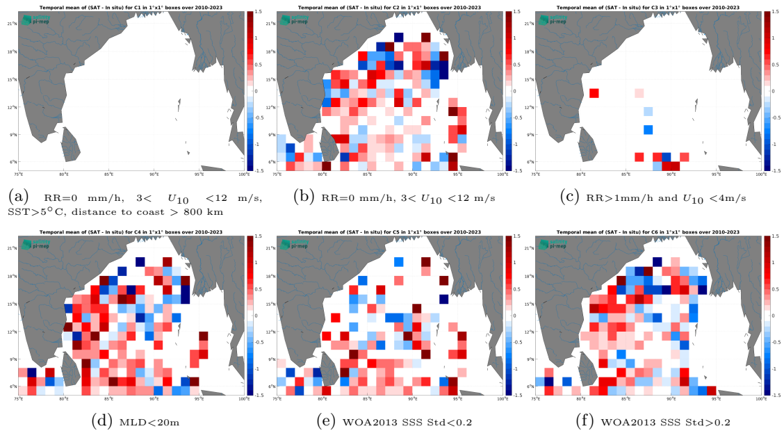
Figure 14: Temporal mean gridded over spatial boxes of size 1^\circ \times 1^\circ of \Delta SSS (SMOS SSS L2 v700 (ESA) - Argo) for 6 different subdatasets corresponding to:RR=0 mm/h, 3 < U_{10} < 12 m/s, SST>5°C, distance to coast > 800 km (a), RR=0 mm/h, 3 < U_{10} < 12 m/s (b), RR>1mm/h and U_{10} < 4 m/s (c),MLD<20m (d),WOA2013 SSS Std<0.2 (e),WOA2013 SSS Std>0.2 (f).
