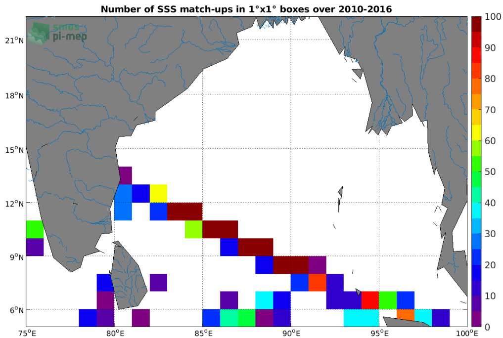
Figure 4: Number of SSS match-ups between TSG (LEGOS-DM) SSS and the SMOS SSS L2 v662 (ESA) SSS product for the Ganga and Brahmaputra river plumes Pi-MEP region over 1^\circ \times 1^\circ boxes and for the full satellite product period.
