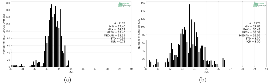
Figure 2: Histograms of SSS from TSG (LEGOS-DM) (a) and SMOS SSS L2 v662 (ESA) (b) considering all match-up pairs per bins of 0.1 over the Ganga and Brahmaputra river plumes Pi-MEP region and for the full satellite product period.
