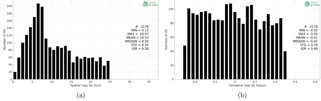
Figure 5: Histograms of the spatial (a) and temporal (b) lags between the location/time of the TSG (LEGOS-DM) measurement and the date of the corresponding SMOS SSS L2 v662 (ESA) SSS pixel.
