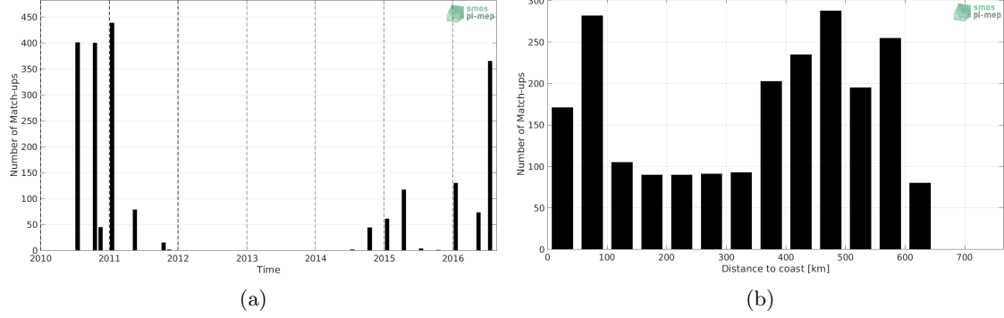
Figure 1: Number of match-ups between TSG (LEGOS-DM) and SMOS SSS L2 v662 (ESA) SSS as a function of time (a) and as function of the distance to coast (b) over the Ganga and Brahmaputra river plumes Pi-MEP region and for the full satellite product period.
