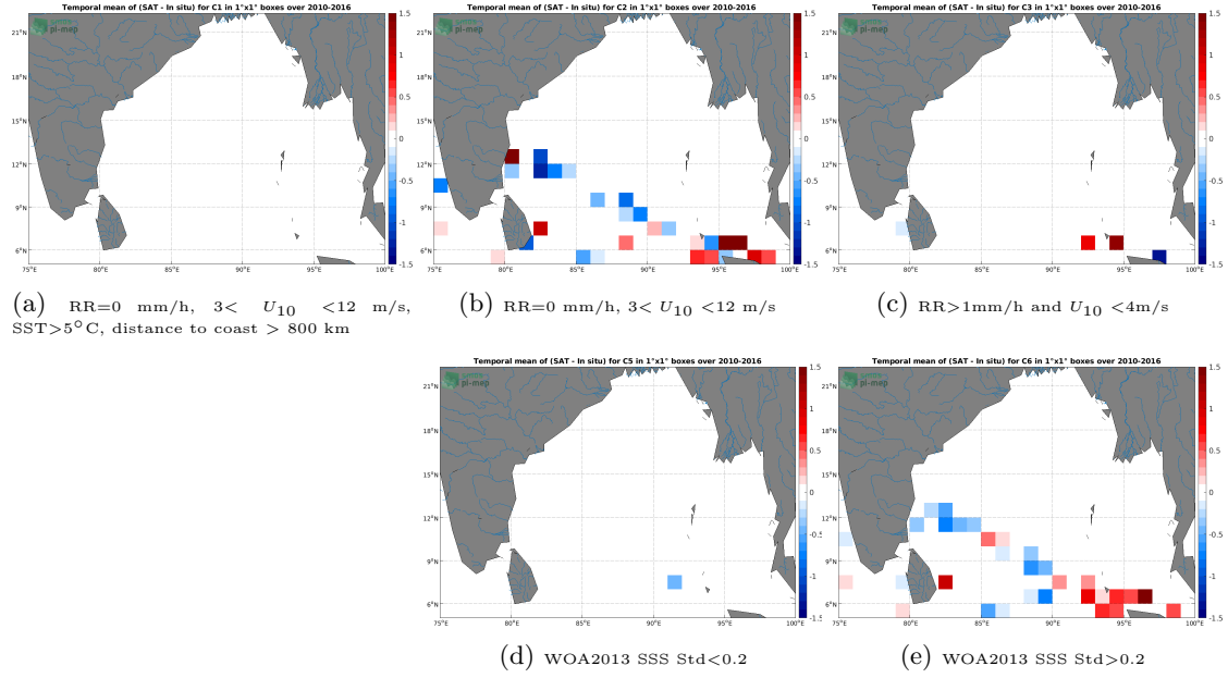
Figure 12: Temporal mean gridded over spatial boxes of size 1^\circ \times 1^\circ of \Delta SSS (SMOS SSS L2 v662 (ESA) - TSG (LEGOS-DM)) for 5 different subdatasets corresponding to:RR=0 mm/h, 3 < U_{10} < 12 m/s, SST >5^\circ C, distance to coast > 800 km (a), RR=0 mm/h, 3 < U_{10} < 12 m/s (b), RR >1 mm/h and U_{10} < 4 m/s (c), WOA2013 SSS Std <0.2 (d), WOA2013 SSS Std >0.2 (e).
