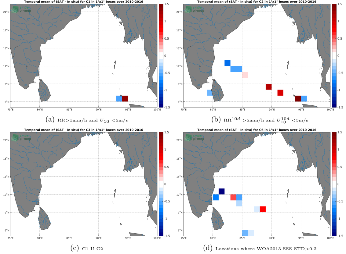
Figure 12: Temporal mean gridded over spatial boxes of size 1^\circ \times 1^\circ of \Delta SSS (SMOS-L2-DPGS-v662 - TSG-LEGOS-DM) for 4 different subdatasets corresponding to: RR > 1\text{mm/h} and U_{10} < 5\text{m/s} (a), RR^{10d} > 5\text{mm/h} and U_{10}^{10d} < 5\text{m/s} (b), C1 U C2 (c), Locations where WOA2013 SSS STD > 0.2 (d).
