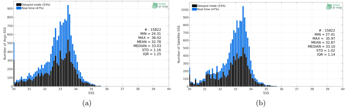
Figure 2: Histograms of SSS from Argo (a) and SMAP SSS L4 OI v1 - 7day (IPRC) (b) considering all match-up pairs per bins of 0.1 over the Ganga and Brahmaputra river plumes Pi-MEP region and for the full satellite product period.
