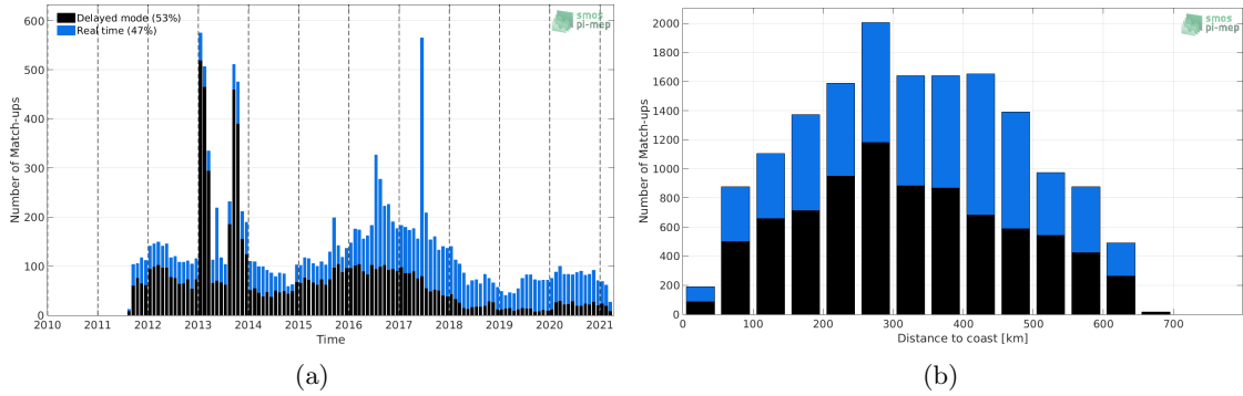
Figure 1: Number of match-ups between Argo and SMAP SSS L4 OI v1 - 7day (IPRC) SSS as a function of time (a) and as function of the distance to coast (b) over the Ganga and Brahmaputra river plumes Pi-MEP region and for the full satellite product period.
