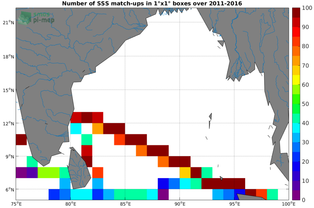
Figure 4: Number of SSS match-ups between TSG (LEGOS-DM) SSS and the SMAP SSS L4 OI v1 - Monthly (IPRC) SSS product for the Ganga and Brahmaputra river plumes Pi-MEP region over 1^\circ \times 1^\circ boxes and for the full satellite product period.
