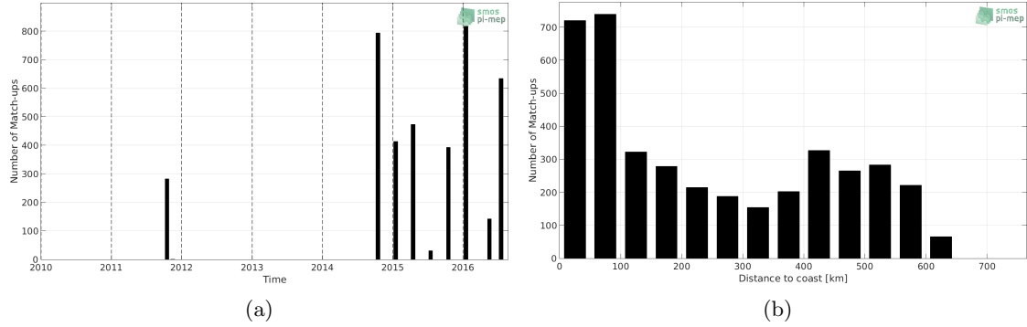
Figure 1: Number of match-ups between TSG (LEGOS-DM) and SMAP SSS L4 OI v1 - Monthly (IPRC) SSS as a function of time (a) and as function of the distance to coast (b) over the Ganga and Brahmaputra river plumes Pi-MEP region and for the full satellite product period.
