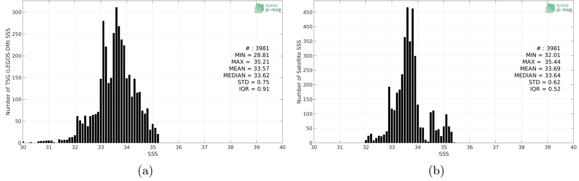
Figure 2: Histograms of SSS from TSG (LEGOS-DM) (a) and SMAP SSS L4 OI v1 - Monthly (IPRC) (b) considering all match-up pairs per bins of 0.1 over the Ganga and Brahmaputra river plumes Pi-MEP region and for the full satellite product period.
