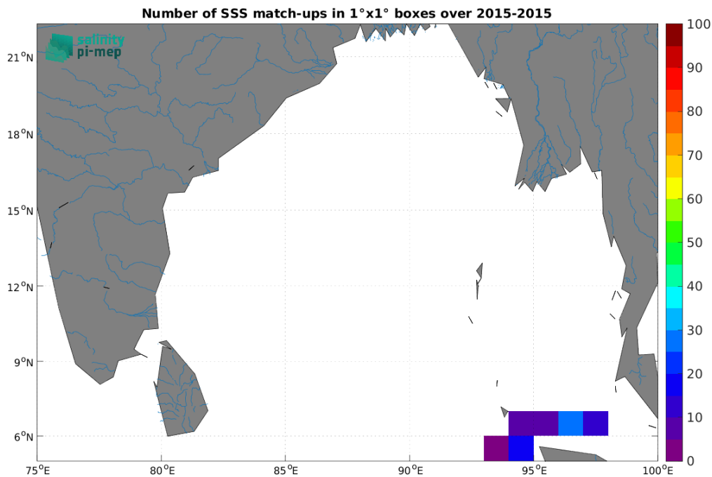
Figure 5: Number of SSS match-ups between TSG (SAMOS) SSS and the SMAP SSS L4 OI v3 - Monthly (ESR) SSS product for the Ganga and Brahmaputra river plumes Pi-MEP region over 1^\circ \times 1^\circ boxes and for the full satellite product period.
