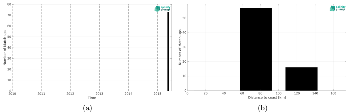
Figure 2: Number of match-ups between TSG (SAMOS) and SMAP SSS L4 OI v3 - Monthly (ESR) SSS as a function of time (a) and as function of the distance to coast (b) over the Ganga and Brahmaputra river plumes Pi-MEP region and for the full satellite product period.
