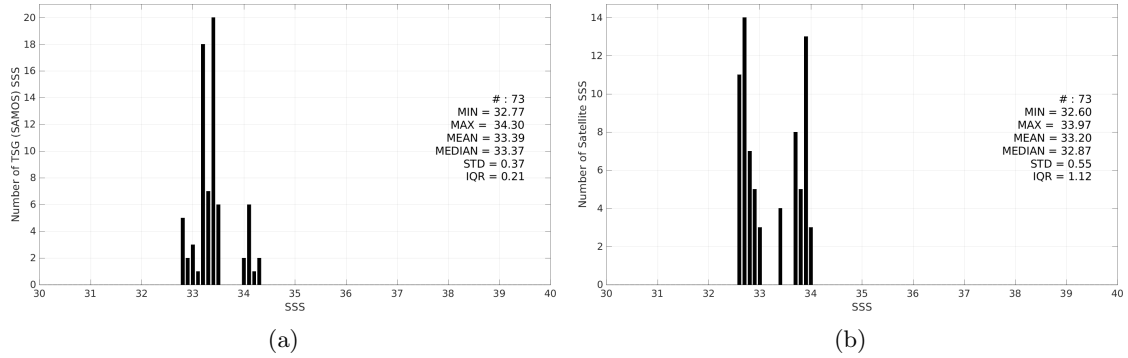
Figure 3: Histograms of SSS from TSG (SAMOS) (a) and SMAP SSS L4 OI v3 - Monthly (ESR) (b) considering all match-up pairs per bins of 0.1 over the Ganga and Brahmaputra river plumes Pi-MEP region and for the full satellite product period.
