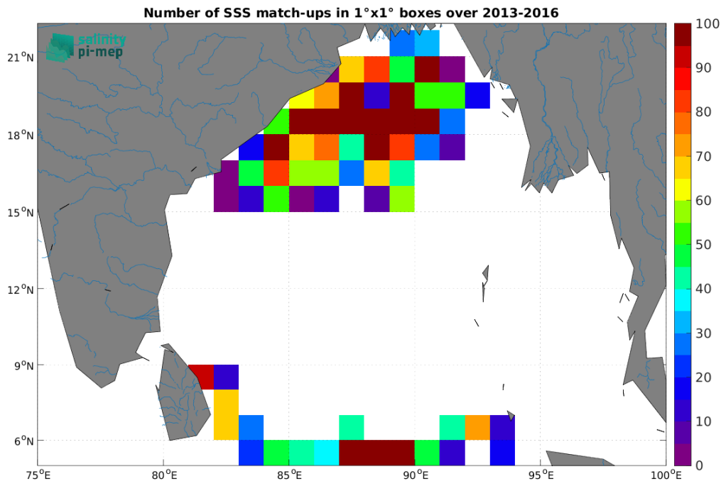
Figure 4: Number of SSS match-ups between Surface drifters SSS and the SMAP SSS L4 OI v3 - Monthly (ESR) SSS product for the Ganga and Brahmaputra river plumes Pi-MEP region over 1^{\circ} \times 1^{\circ} boxes and for the full satellite product period.
