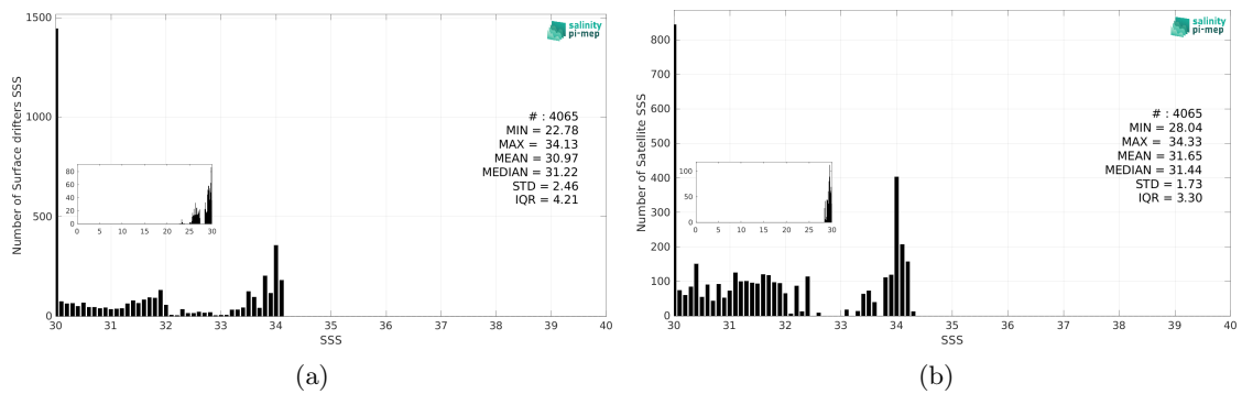
Figure 3: Histograms of SSS from Surface drifters (a) and SMAP SSS L4 OI v3 - Monthly (ESR) (b) considering all match-up pairs per bins of 0.1 over the Ganga and Brahmaputra river plumes Pi-MEP region and for the full satellite product period.
