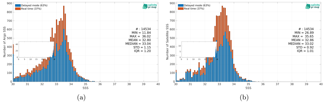
Figure 3: Histograms of SSS from Argo (a) and SMAP SSS L4 OI v3 - Monthly (ESR) (b) considering all match-up pairs per bins of 0.1 over the Ganga and Brahmaputra river plumes Pi-MEP region and for the full satellite product period.
