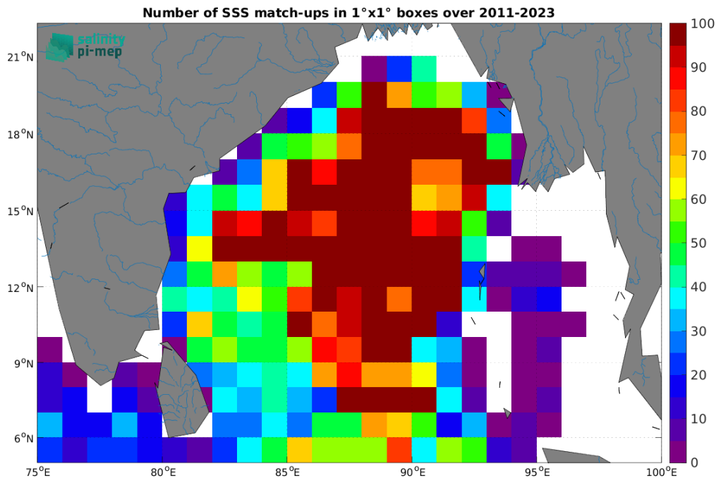
Figure 5: Number of SSS match-ups between Argo SSS and the SMAP SSS L4 OI v3 - Monthly (ESR) SSS product for the Ganga and Brahmaputra river plumes Pi-MEP region over 1^\circ \times 1^\circ boxes and for the full satellite product period.
