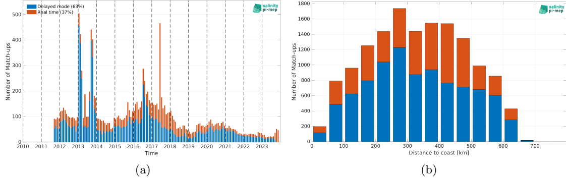
Figure 2: Number of match-ups between Argo and SMAP SSS L4 OI v3 - Monthly (ESR) SSS as a function of time (a) and as function of the distance to coast (b) over the Ganga and Brahmaputra river plumes Pi-MEP region and for the full satellite product period.
