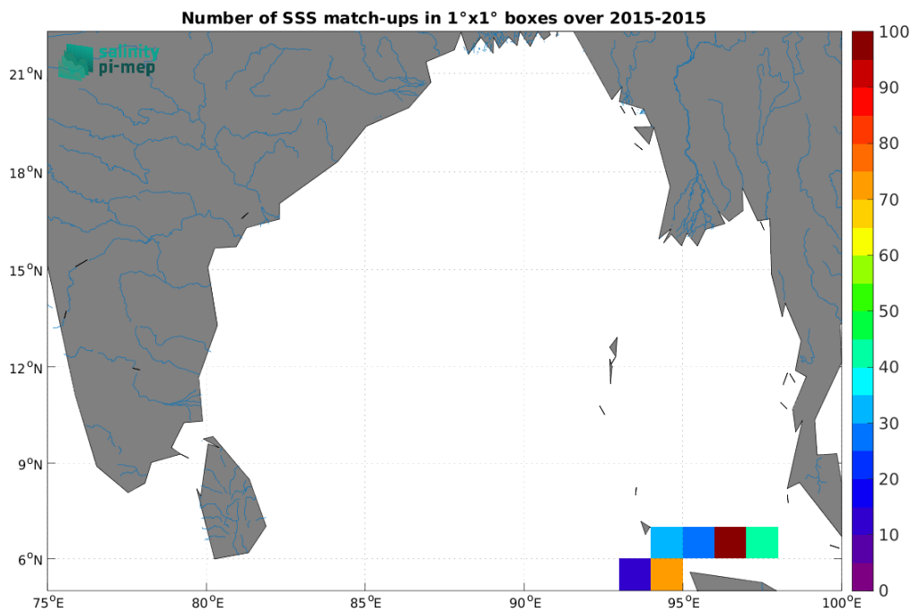
Figure 5: Number of SSS match-ups between TSG (SAMOS) SSS and the SMAP SSS L4 OI v3 - Daily (ESR) SSS product for the Ganga and Brahmaputra river plumes Pi-MEP region over 1^\circ \times 1^\circ boxes and for the full satellite product period.
