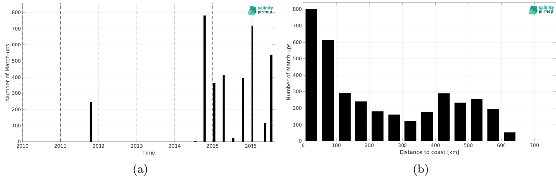
Figure 2: Number of match-ups between TSG (LEGOS-DM) and SMAP SSS L4 OI v3 - Daily (ESR) SSS as a function of time (a) and as function of the distance to coast (b) over the Ganga and Brahmaputra river plumes Pi-MEP region and for the full satellite product period.
