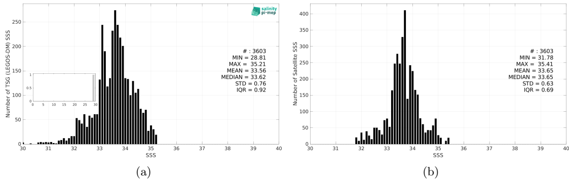
Figure 3: Histograms of SSS from TSG (LEGOS-DM) (a) and SMAP SSS L4 OI v3 - Daily (ESR) (b) considering all match-up pairs per bins of 0.1 over the Ganga and Brahmaputra river plumes Pi-MEP region and for the full satellite product period.
