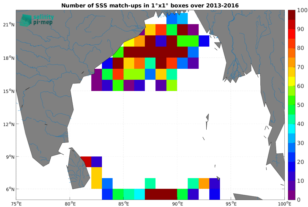
Figure 4: Number of SSS match-ups between Surface drifters SSS and the SMAP SSS L4 OI v3 - Daily (ESR) SSS product for the Ganga and Brahmaputra river plumes Pi-MEP region over 1^\circ \times 1^\circ boxes and for the full satellite product period.
