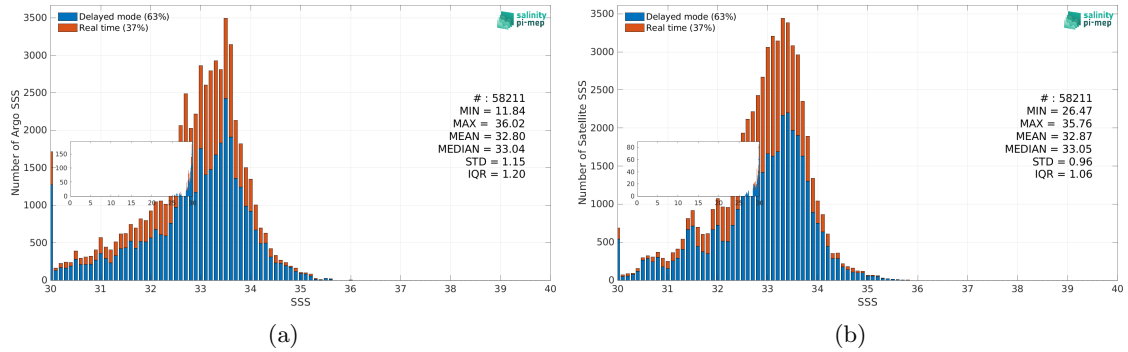
Figure 3: Histograms of SSS from Argo (a) and SMAP SSS L4 OI v3 - Daily (ESR) (b) considering all match-up pairs per bins of 0.1 over the Ganga and Brahmaputra river plumes Pi-MEP region and for the full satellite product period.
