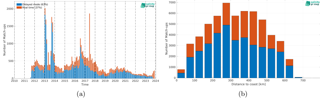
Figure 2: Number of match-ups between Argo and SMAP SSS L4 OI v3 - Daily (ESR) SSS as a function of time (a) and as function of the distance to coast (b) over the Ganga and Brahmaputra river plumes Pi-MEP region and for the full satellite product period.
