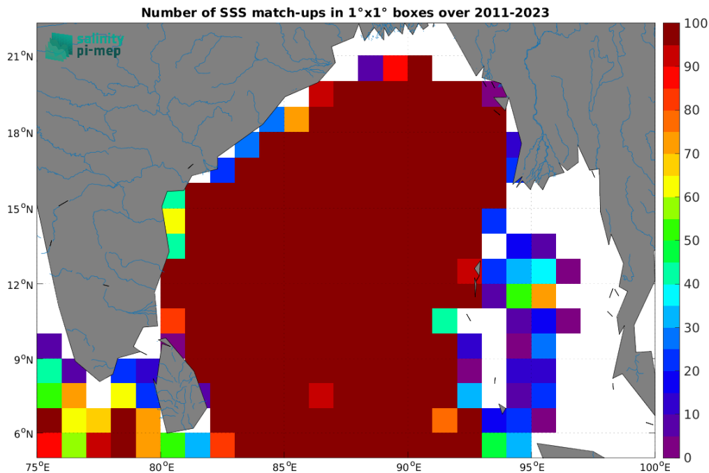
Figure 5: Number of SSS match-ups between Argo SSS and the SMAP SSS L4 OI v3 - Daily (ESR) SSS product for the Ganga and Brahmaputra river plumes Pi-MEP region over 1^\circ \times 1^\circ boxes and for the full satellite product period.
