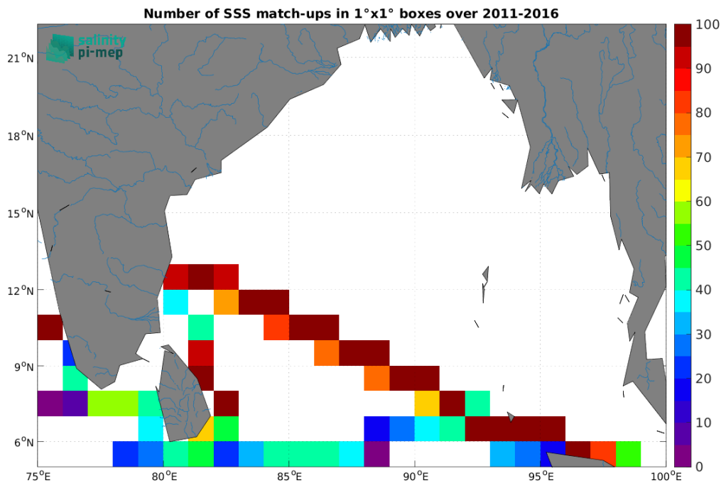
Figure 4: Number of SSS match-ups between TSG (LEGOS-DM) SSS and the SMAP SSS L4 OI v2 - Monthly (IPRC) SSS product for the Ganga and Brahmaputra river plumes Pi-MEP region over 1^\circ \times 1^\circ boxes and for the full satellite product period.
