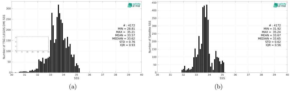
Figure 2: Histograms of SSS from TSG (LEGOS-DM) (a) and SMAP SSS L4 OI v2 - Monthly (IPRC) (b) considering all match-up pairs per bins of 0.1 over the Ganga and Brahmaputra river plumes Pi-MEP region and for the full satellite product period.
