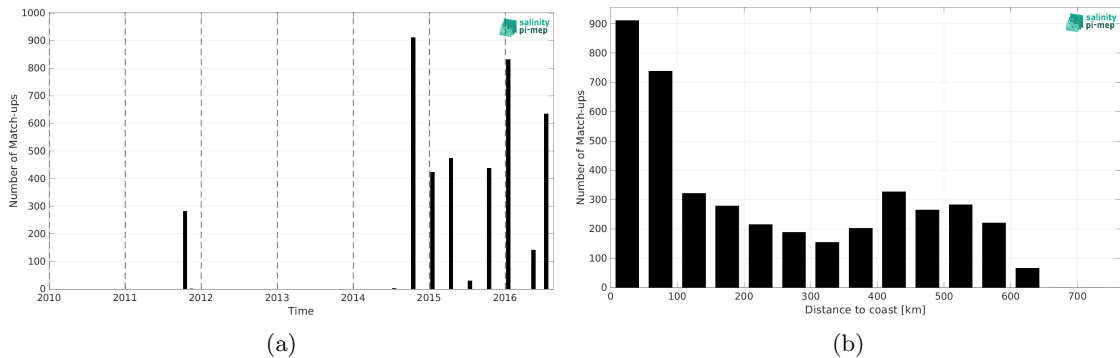
Figure 1: Number of match-ups between TSG (LEGOS-DM) and SMAP SSS L4 OI v2 - Monthly (IPRC) SSS as a function of time (a) and as function of the distance to coast (b) over the Ganga and Brahmaputra river plumes Pi-MEP region and for the full satellite product period.
