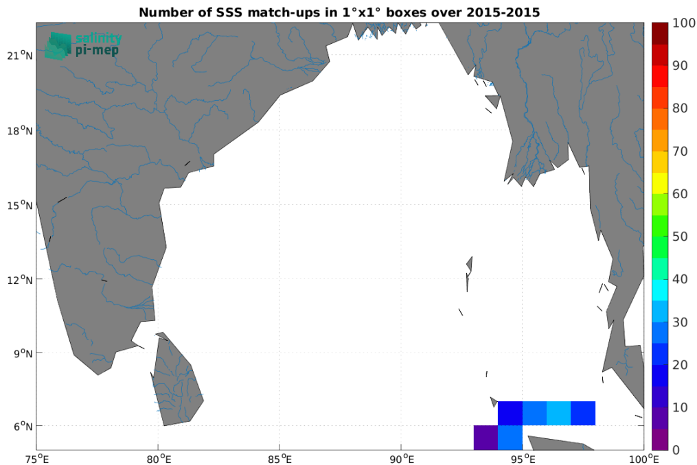
Figure 5: Number of SSS match-ups between TSG (SAMOS) SSS and the SMAP SSS L3 v6 - 8-Day running (RSS) SSS product for the Ganga and Brahmaputra river plumes Pi-MEP region over 1°x1° boxes and for the full satellite product period.
