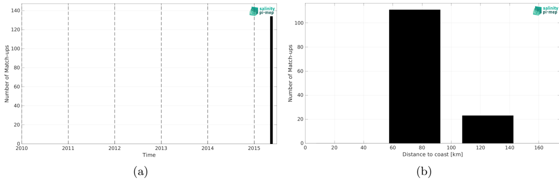
Figure 2: Number of match-ups between TSG (SAMOS) and SMAP SSS L3 v6 - 8-Day running (RSS) SSS as a function of time (a) and as function of the distance to coast (b) over the Ganga and Brahmaputra river plumes Pi-MEP region and for the full satellite product period.
