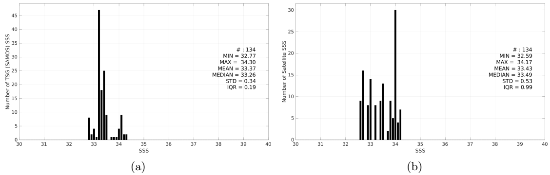
Figure 3: Histograms of SSS from TSG (SAMOS) (a) and SMAP SSS L3 v6 - 8-Day running (RSS) (b) considering all match-up pairs per bins of 0.1 over the Ganga and Brahmaputra river plumes Pi-MEP region and for the full satellite product period.
