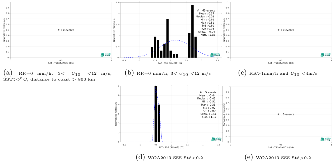
Figure 15: Normalized histogram of \Delta SSS (SMAP SSS L3 v6 - 8-Day running (RSS) - TSG (SAMOS)) for 5 different subdatasets corresponding to: RR=0 mm/h, 3 < U_{10} < 12 m/s, SST >5^{\circ} C, distance to coast > 800 km (a), RR=0 mm/h, 3 < U_{10} < 12 m/s (b), RR >1 mm/h and U_{10} < 4 m/s (c), WOA2013 SSS Std <0.2 (d), WOA2013 SSS Std >0.2 (e).
