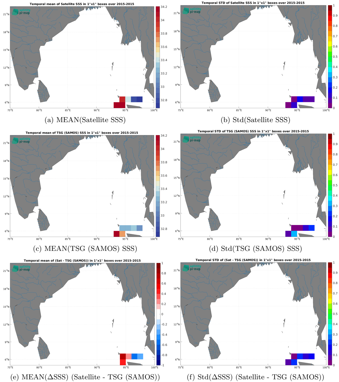
Figure 7: Temporal mean (left) and Std (right) of SSS from SMAP SSS L3 v6 - Monthly (RSS) (top), TSG (SAMOS) (middle), and of \Delta SSS (Satellite - TSG (SAMOS)). Only match-up pairs are used to generate these maps.
