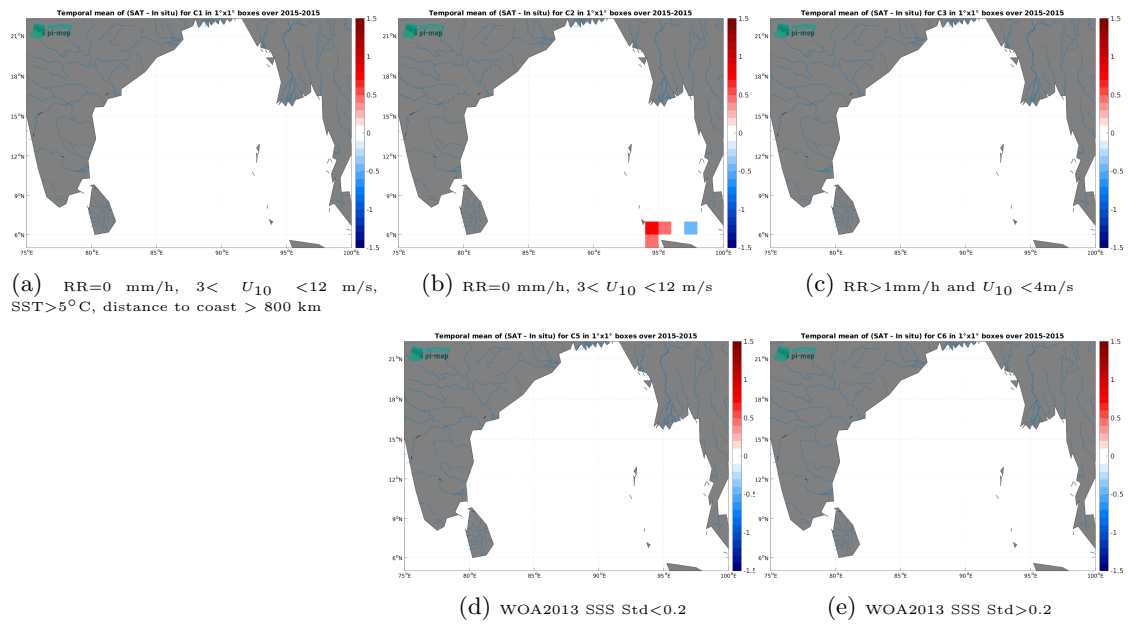
Figure 14: Temporal mean gridded over spatial boxes of size 1^\circ \times 1^\circ of \Delta SSS (SMAP SSS L3 v6 - Monthly (RSS) - TSG (SAMOS)) for 5 different subdatasets corresponding to:RR=0 mm/h, 3 < U_{10} < 12 m/s, SST>5°C, distance to coast > 800 km (a), RR=0 mm/h, 3 < U_{10} < 12 m/s (b), RR>1mm/h and U_{10} < 4 m/s (c), WOA2013 SSS Std<0.2 (d), WOA2013 SSS Std>0.2 (e).
