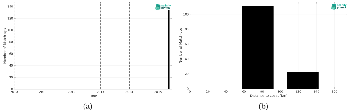
Figure 2: Number of match-ups between TSG (SAMOS) and SMAP SSS L3 v6 - Monthly (RSS) SSS as a function of time (a) and as function of the distance to coast (b) over the Ganga and Brahmaputra river plumes Pi-MEP region and for the full satellite product period.
