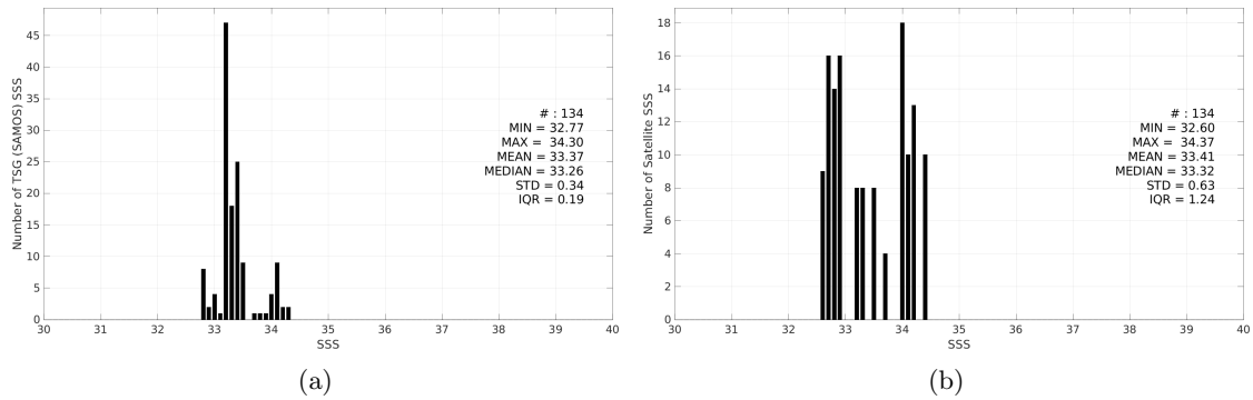
Figure 3: Histograms of SSS from TSG (SAMOS) (a) and SMAP SSS L3 v6 - Monthly (RSS) (b) considering all match-up pairs per bins of 0.1 over the Ganga and Brahmaputra river plumes Pi-MEP region and for the full satellite product period.
