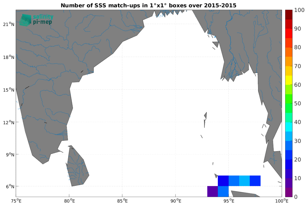
Figure 5: Number of SSS match-ups between TSG (SAMOS) SSS and the SMAP SSS L3 v6 - Monthly (RSS) SSS product for the Ganga and Brahmaputra river plumes Pi-MEP region over 1^{\circ} \times 1^{\circ} boxes and for the full satellite product period.
