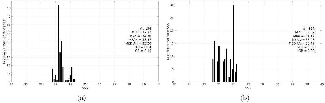
Figure 3: Histograms of SSS from TSG (SAMOS) (a) and SMAP SSS L3 v5.3 - 8-Day running (RSS) (b) considering all match-up pairs per bins of 0.1 over the Ganga and Brahmaputra river plumes Pi-MEP region and for the full satellite product period.
