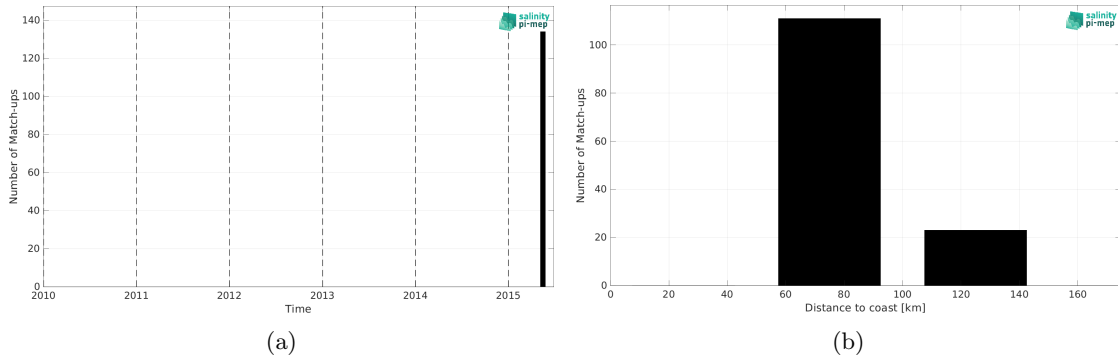
Figure 2: Number of match-ups between TSG (SAMOS) and SMAP SSS L3 v5.3 - 8-Day running (RSS) SSS as a function of time (a) and as function of the distance to coast (b) over the Ganga and Brahmaputra river plumes Pi-MEP region and for the full satellite product period.
