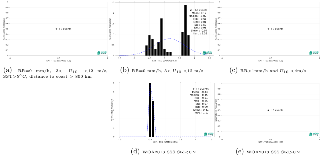
Figure 15: Normalized histogram of \Delta SSS (SMAP SSS L3 v5.3 - 8-Day running (RSS) - TSG (SAMOS)) for 5 different subdatasets corresponding to: RR=0 mm/h, 3 < U_{10} < 12 m/s, SST > 5^{\circ}\text{C} , distance to coast > 800 km (a), RR=0 mm/h, 3 < U_{10} < 12 m/s (b), RR > 1 mm/h and U_{10} < 4 m/s (c), WOA2013 SSS Std < 0.2 (d), WOA2013 SSS Std > 0.2 (e).
